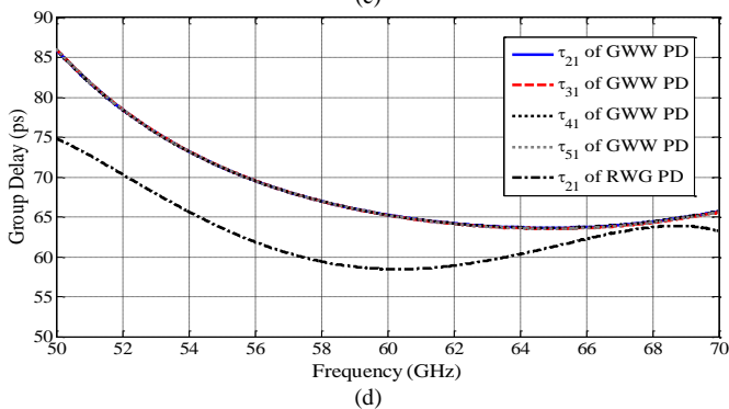
Fig. 8. (a) Simulation results for amplitudes of reflection and transmission coefficients, (b) phase difference of outputs (c) electric field distribution at frequency 60 GHz and (d) group delay variation for the 4-way H-shaped GGW power divider in comparison with ordinary rectangular WG power divider.
