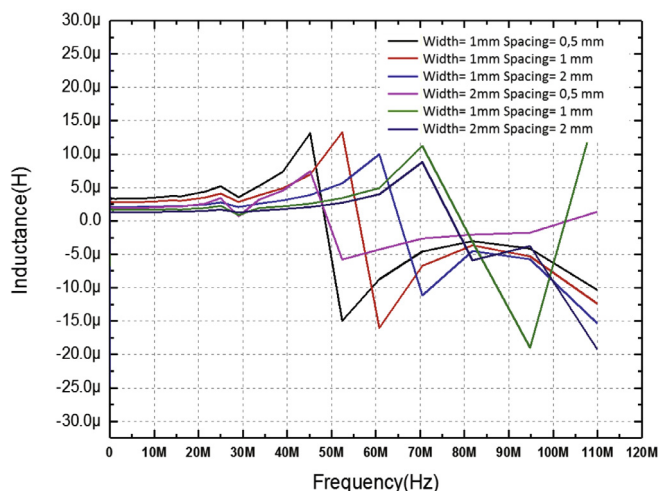
FIGURE 5 Equivalent inductance vs. frequency measured for six NFC coils of graphene paper with different geometrical parameters using a HP 4294A Impedance Analyser.
