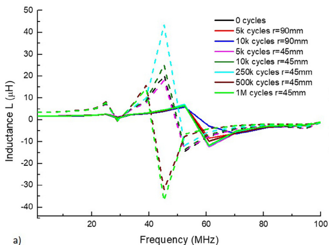
FIGURE 6 (a) Equivalent inductance and (b) electrical resistance of a commercial metallic antenna (dashed lines) and of graphene paper antenna (solid lines) vs frequency upon bending up to 1 million cycles at different bending radii r . Inset: picture of the bending test set-up.
