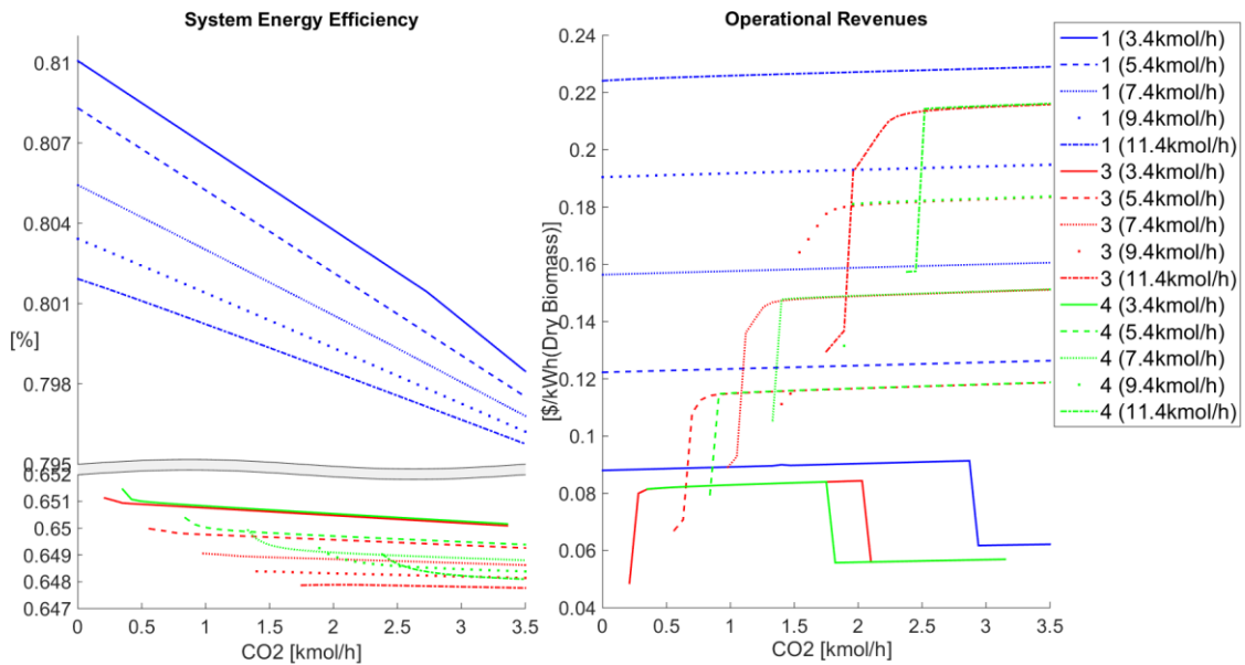
Figure 12. Total system energy efficiency and operating revenues as a function of CO 2 feed. The line colors correspondent to different configurations and the line types correspond to the amounts of H 2 feed.
