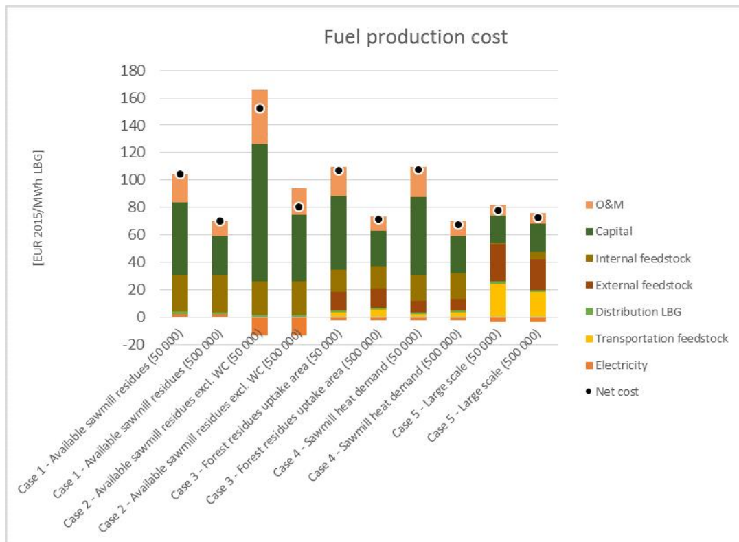
Figure 14. Fuel production cost (FPC) for all cases and the 50 000 and 500 000 m³/yr sawmill sizes.
