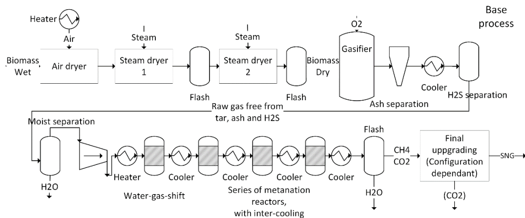
Figure 4. Overview flowchart of the direct gasification process used for the power-to-gas concept.
