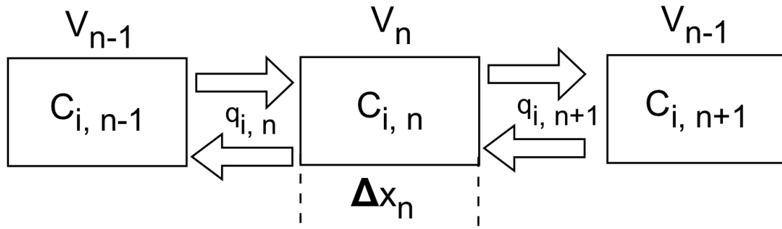
Figure 11. Neighboring volume elements (length \Delta x_n ) of the numeric model q_{i,n} are the fluxes and C_{i,n} are the concentrations accumulated over time due to those fluxes.
