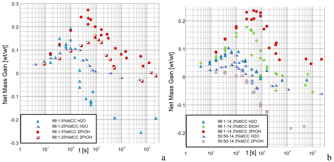
Figure 17. NMG as a function of time. The two stages of initial nonsolvent absorption during coagulation and secondary mass-loss during washout are displayed.
