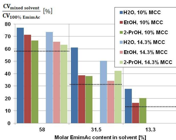
Figure 13. Ratios of CVs (wt%) for solutions in mixed solvents relative to the pure [C_2mim][OAc] solutions at equal cellulose concentration.
