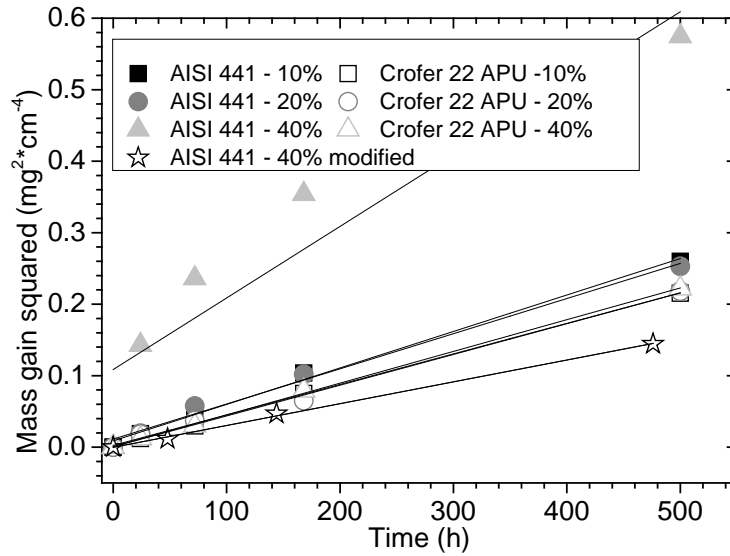
Figure 3. Mass gain squared plotted against time for AISI 441 and Crofer 22 APU in all tested atmospheres. The star-shaped data markers represent the mass gain of AISI 441 exposed to 40% H 2 O, where the mass gain after the first 24 h of time was subtracted in order to evaluate if parabolic oxidation takes place after 24 h for AISI 441 in 40% H 2 O.
