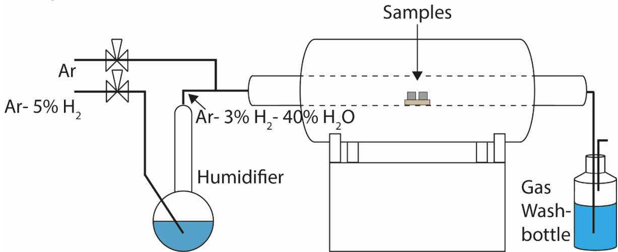
Figure 1. Schematic drawing of the experimental setup used.
