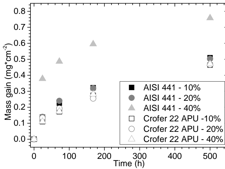
Figure 2. Mass gain plotted against time for AISI 441 and Crofer 22 APU in all tested atmospheres.
