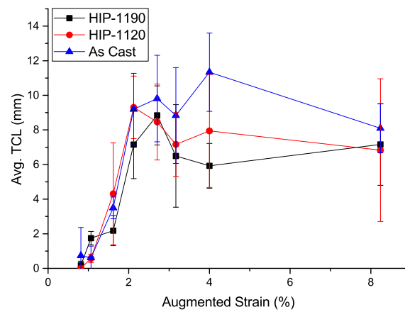
Figure 9. FZ cracking response with standard deviations for the as-cast, HIP-1120 and HIP-1190 conditions
