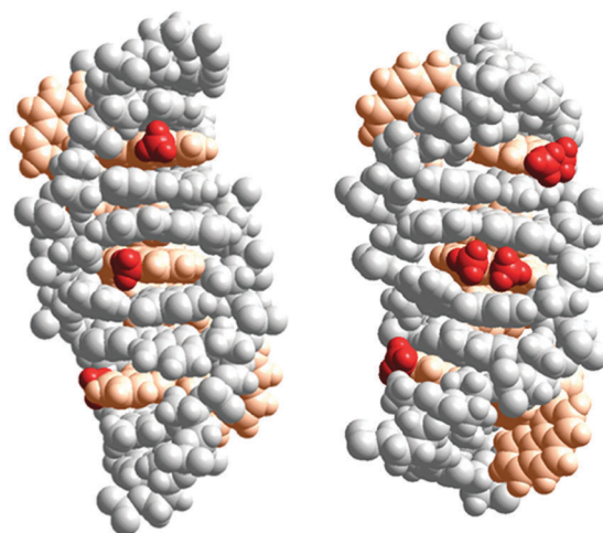
Fig. 4 Schematic illustration of the proposed interaction geometries for \Delta -2 (left) and \Delta -3 (right) intercalated into DNA. The model was constructed by manual docking and subsequent energy minimization in vacuum, using the Amber 2 force field in the HyperChem 8.0 software package (HyperCube, Inc.). The ruthenium(II) ions together with the ancillary and intercalating ligands are colored orange, while the methyl substituents are colored red for easier identification.
