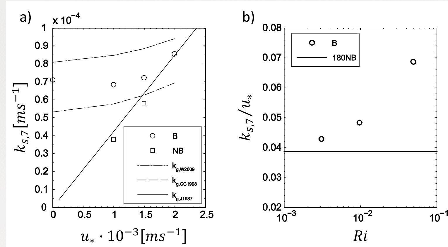
Figure 2. a) The scalar transfer velocity k_{s,7} = k_{s,7}/\Delta s_{s,7} . Circles denote cases with buoyancy and squares denote no-buoyancy cases. The dashed and dash-dotted lines denote the wind parameterizations with n = 1/2 according to equations (3) and (4) respectively. The solid line denotes a linear increase of the transfer velocity as a function of the friction velocity (2). b) Transfer velocity constant k_{s,7}/u_* as a function of Ri .
