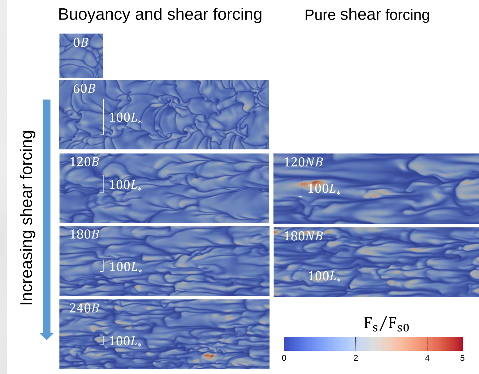
Figure 1. Normalized surface-normal scalar flux fields. The cases are named as the Re_* = (u_* v)/H and B for Buoyancy and NB for No-Buoyancy. The same scaling is used for all subplots. The length scale 100L_* , where L_* = v/u_* , is indicated in the subplots for cases with u_* > 0 .
