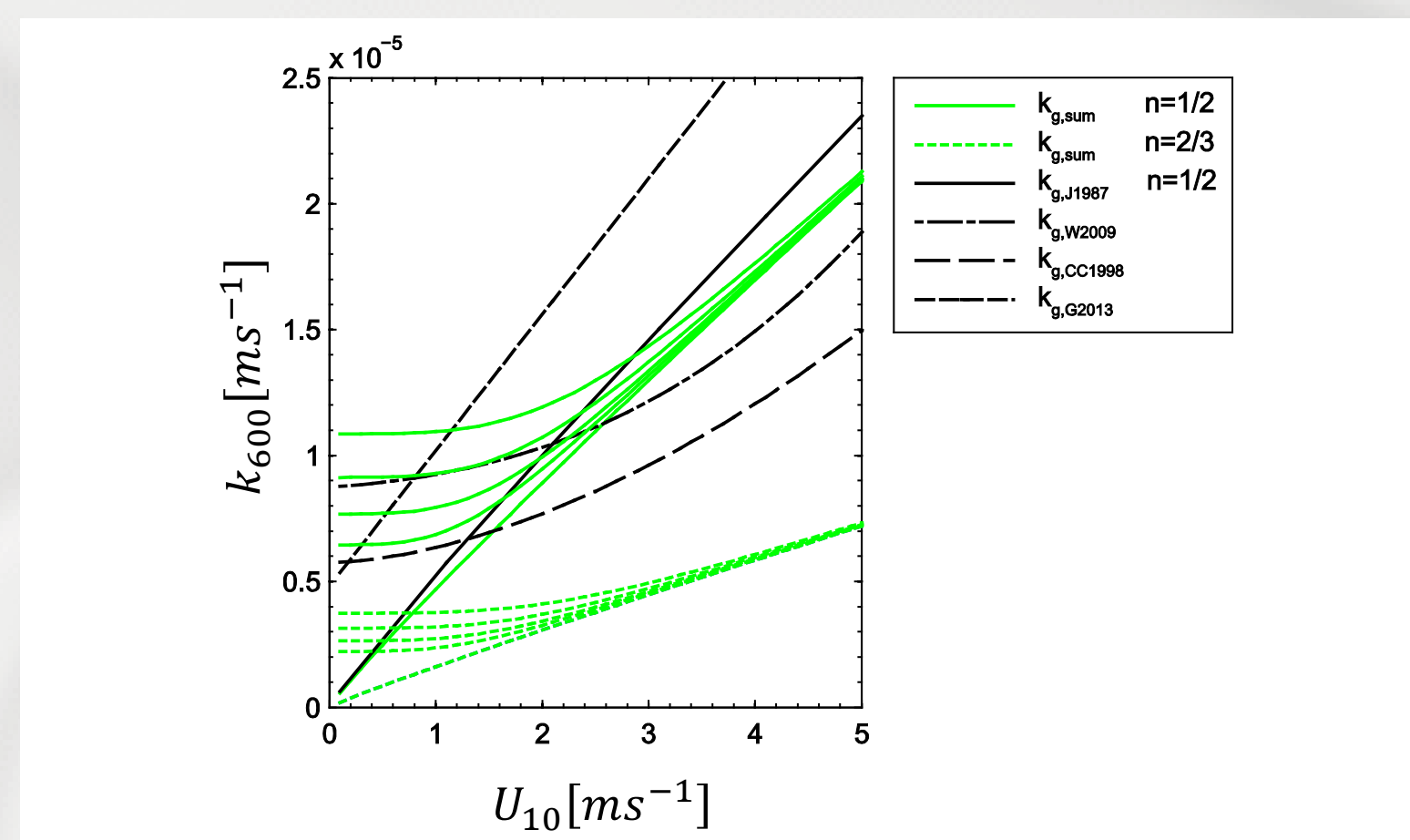
Figure 3. Transfer velocity constant k_{g,600} according to equation (23) in green for Q_0 = 0, 50, 100, 200 and 400 \text{ W m}^{-2} and n = 1/2 (clean) and dotted line n = 2/3 (saturated surfactant). The parametrizations in equations (2-5) are given for reference. The transfer velocity estimated with equation (4) is transformed into Sc = 600 using k_{g,Sc_1} = k_{g,Sc_2} (Sc_1/Sc_2)^{-n} and n = 1/2 .
