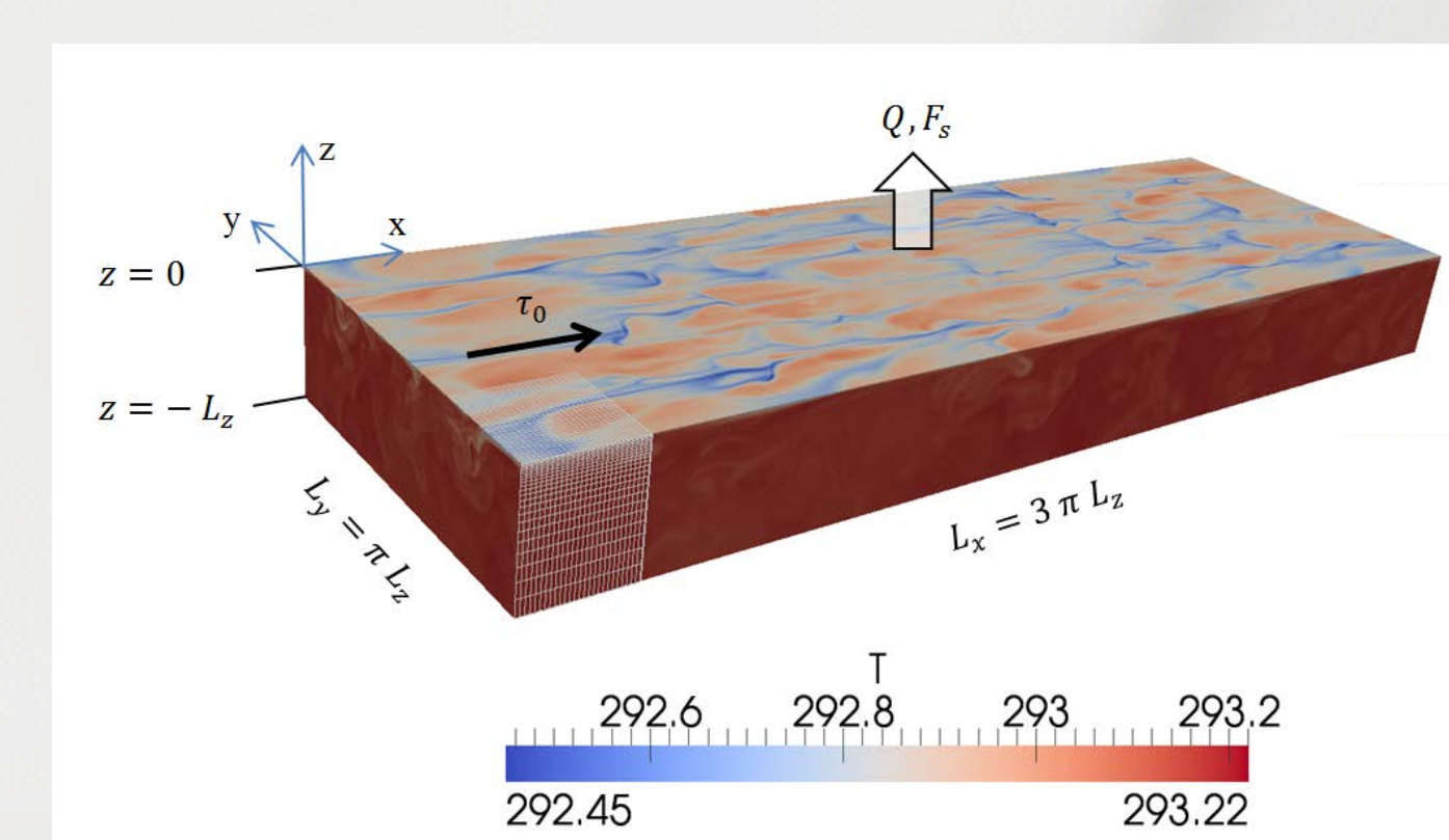
Figure 4. Computational domain for the cases with combined buoyancy and shear stress forcing. The domain size is given by L_z = 0.1204 \text{ m} , L_x = 3\pi L_z and L_y = \pi L_z in the depth, streamwise, and spanwise direction, respectively. The surface is subject to a constant outward-going heat flux, Q_0 , and a constant scalar concentration, S_0 , while the bottom is subject to zero flux boundary conditions. The velocity boundary conditions are either slip, no-slip or constant shear stress, \tau_0 , at the surface boundary and slip at the bottom boundary. Periodic (cyclic) boundary conditions are used for all variables in the horizontal ( x - and y -) directions.
