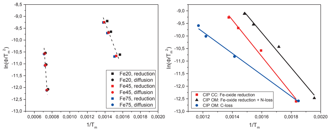
Figure 16: Kinetic plots for a) water-atomized and b) carbonyl iron powder.
