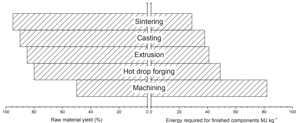
Figure 1: Raw material yield and energy consumption compared for some manufacturing methods. Redrawn from [1].
