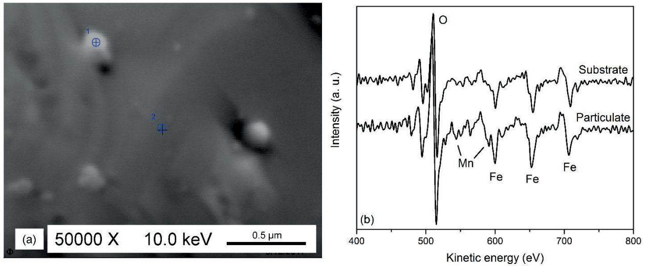
Figure 12: AES analysis providing information about the surface chemical state difference between a surface feature that is a particulate oxide, and the surrounding powder particle surface.
