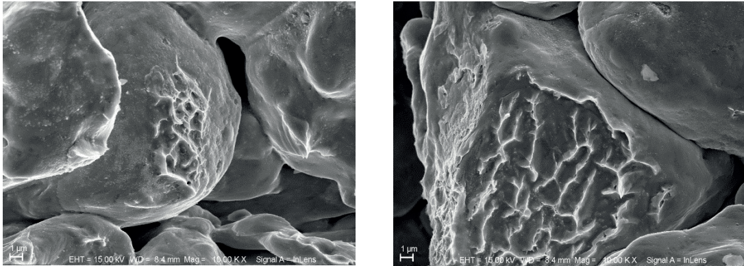
Figure 19: Fracture surfaces of compacts sintered at 700 °C, a) 400 MPa, b) 800 MPa.
