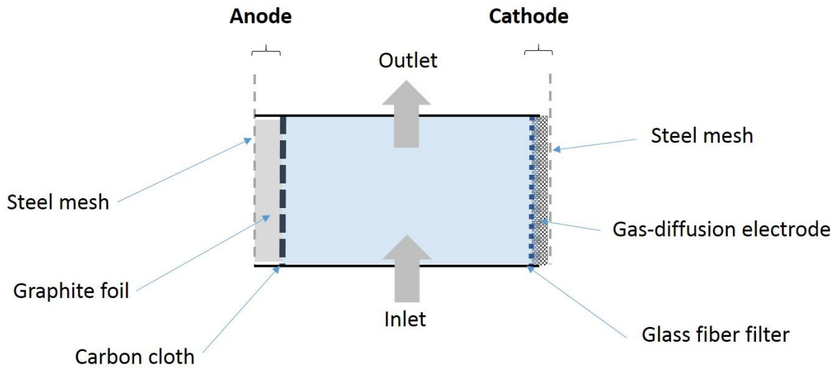
Figure 4. Schematic of the MFCs set-up.
