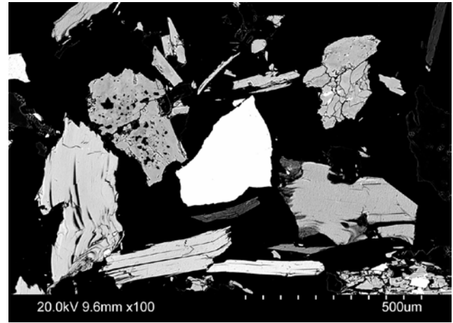
Figure 32. Backscattered electron image of a scheelite liberated particle of W2 after IPB at 0.20.
