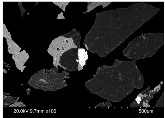
Figure 18. Backscattered electron image of a composite particle of W1 after IPB at 0.30. The particle is embedded in by scheelite in apatite.
