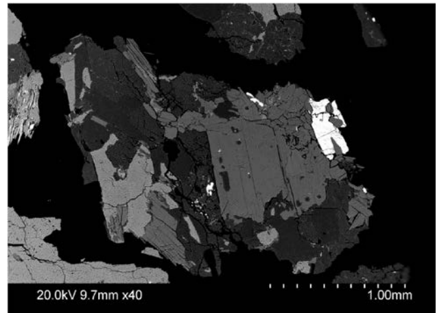
Figure 16. Backscattered electron image of a composite particle of W1 after IPB at 0.10. The particle is embedded in by scheelite and K-feldspar.
