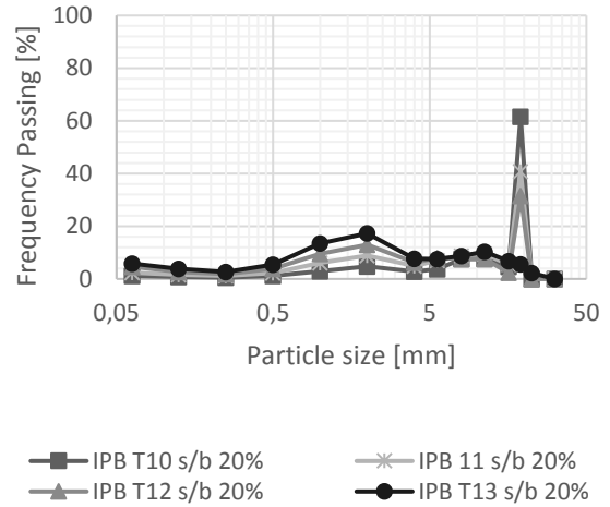
Figure 43. Product particle size distributions for the IPB 20% test series (frequency) for T4.
