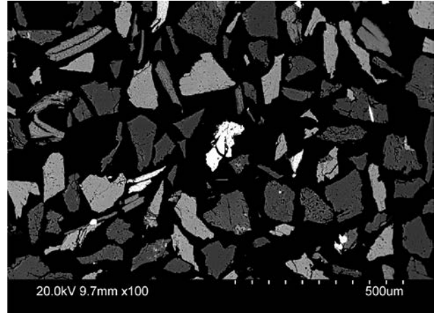
Figure 24. Backscattered electron image of a wolframite liberated particle of W2 after IPB at 0.10.
