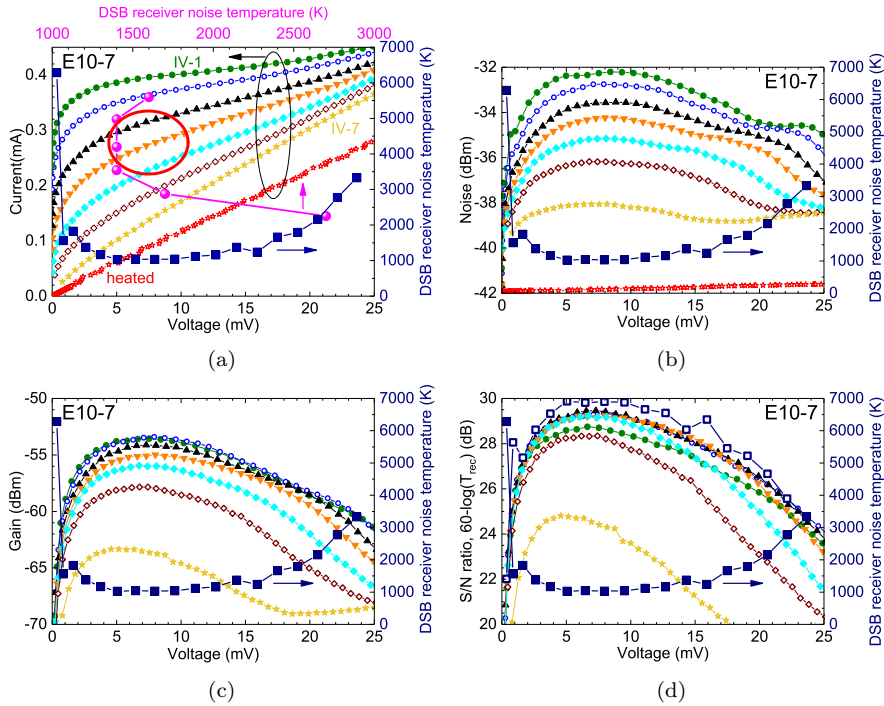
Fig. 6.14: HEB E10-7 with 0.69 THz LO pumping and at 5 K. The area of the highest S/N ratio is marked on the I-V plane. ( Data adopted from [Paper H] )
