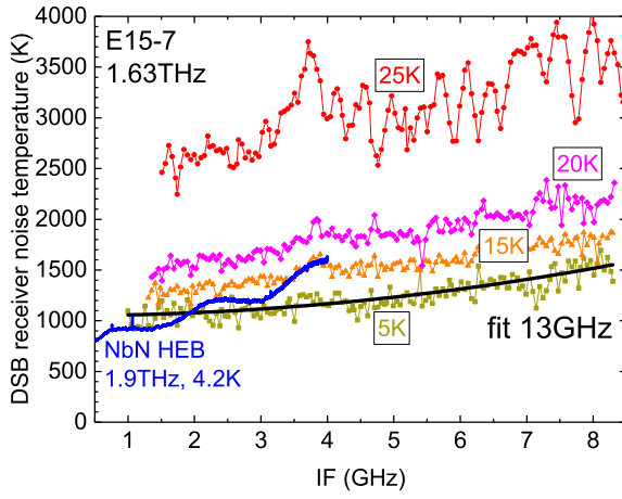
Fig. 6.18: HEB E15-7 receiver noise temperature (at 1.63 THz) versus the IF recorded at 5 K, 15 K, 20 K, and 25 K. The NbN HEB mixer data is from Ref. [32].
