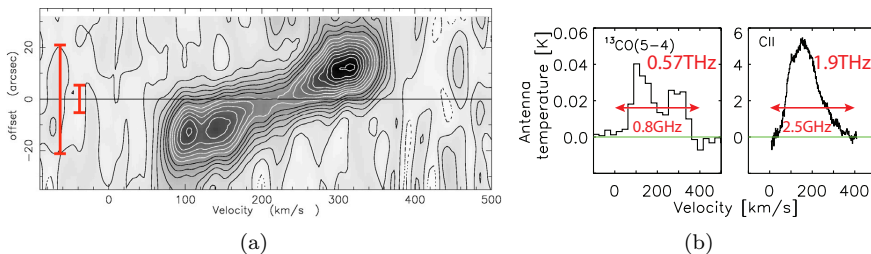
Fig. 1.2: Observation of Galaxy M82 by the Herschel Space Observatory (a) Position-velocity diagram of the Nucleus of M82. The two red bars show the largest (44'' at 0.57 THz) and the smallest (12'' at 1.9 THz) beams in observations. (b) Observed spectra of Galaxy M82: CO line at 0.57 THz by SIS mixers (left) and CII line at 1.9 THz by HEB mixers (right). The same velocity range corresponds to about three times wider signal bandwidth at 1.9 THz than at 0.57 THz. Illustrations from Ref. [43].
