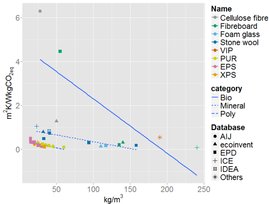
Figure 4.2: Correlation between material density and eco-efficiency of materials in GWP from multiple data sources
