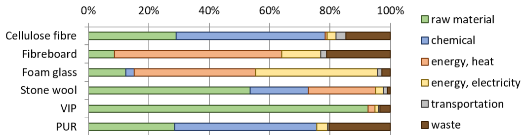
Figure 4.1: Composition of raw material, transportation and energy on the environmental impact of each thermal insulation material on ReCiPe in A1-C4 module
