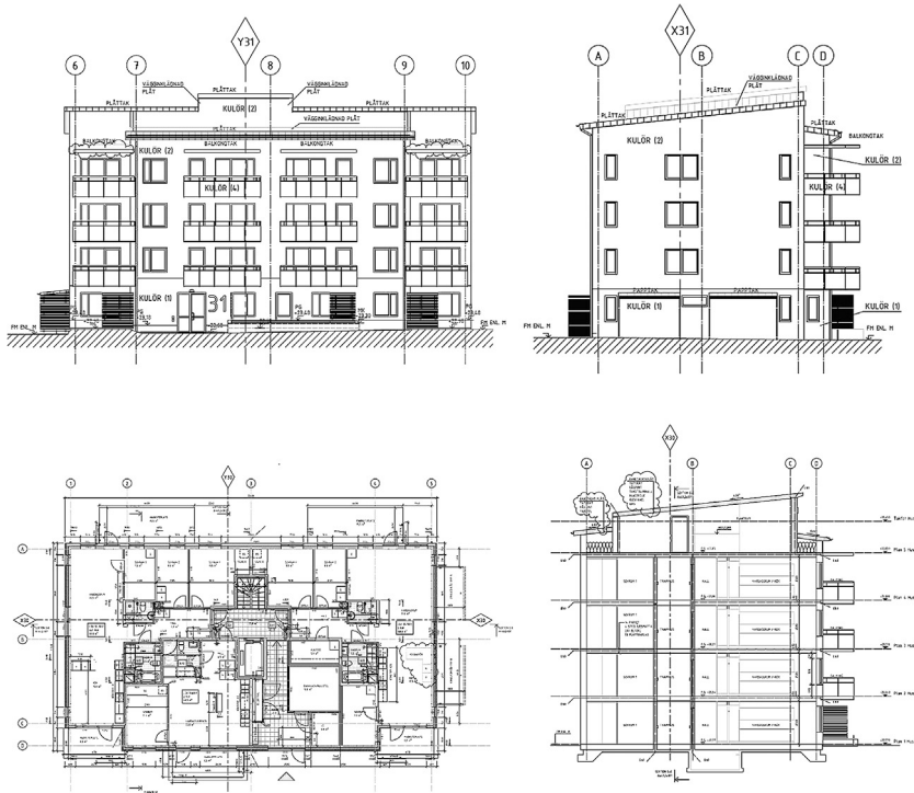
Fig. 2. Drawings of the base house (Skanska).
