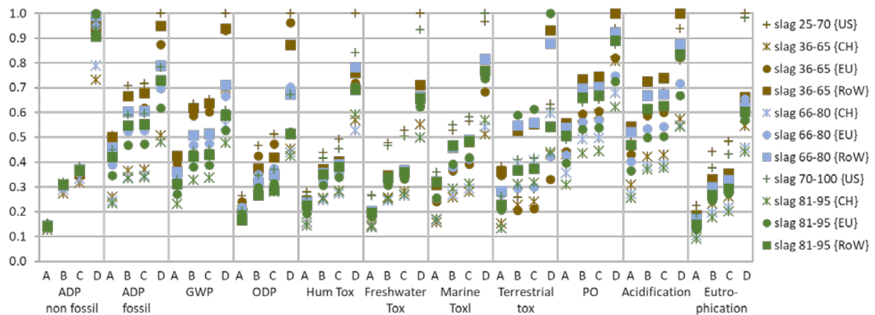
Figure 5. Normalized life cycle environmental impact of green concretes. The shape represents the geographic representation and the color represents the slag content of the green concrete
