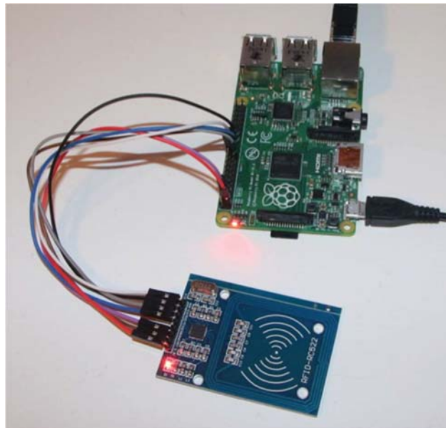
Figure 12: A Raspberry Pi with an RFID reader (MFRC522 board) attached (paper II).
