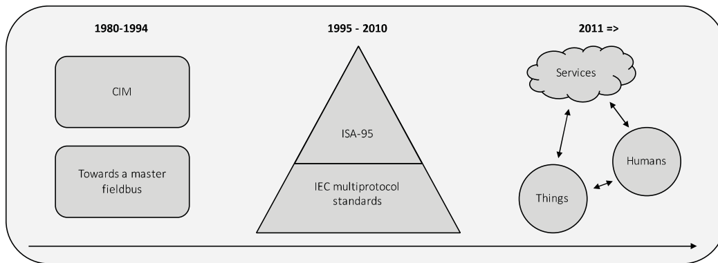
Figure 8: History of principle architecture of shop floor IT since 1980.
