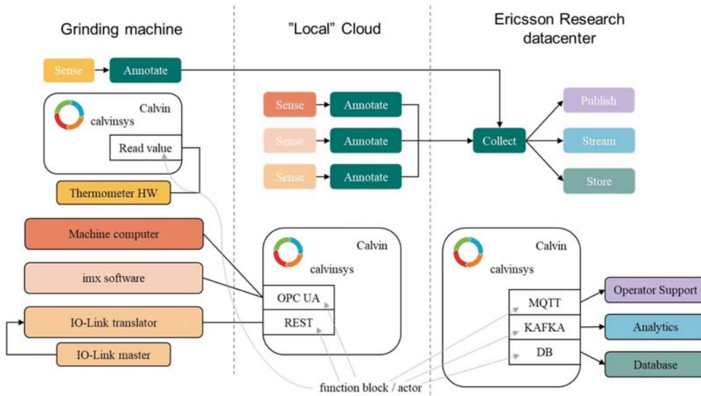
Figure 19: The Calvin application. It is distributed over three physical locations: The Raspberry Pi, the local cloud, and the centralised cloud.
