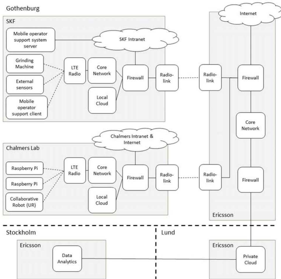
Figure 18: The connectivity infrastructure of the 5GEM project. Visualises how different technologies are connected from the SKF factory and Chalmers laboratory to Ericsson's cloud and data analytics centre.
