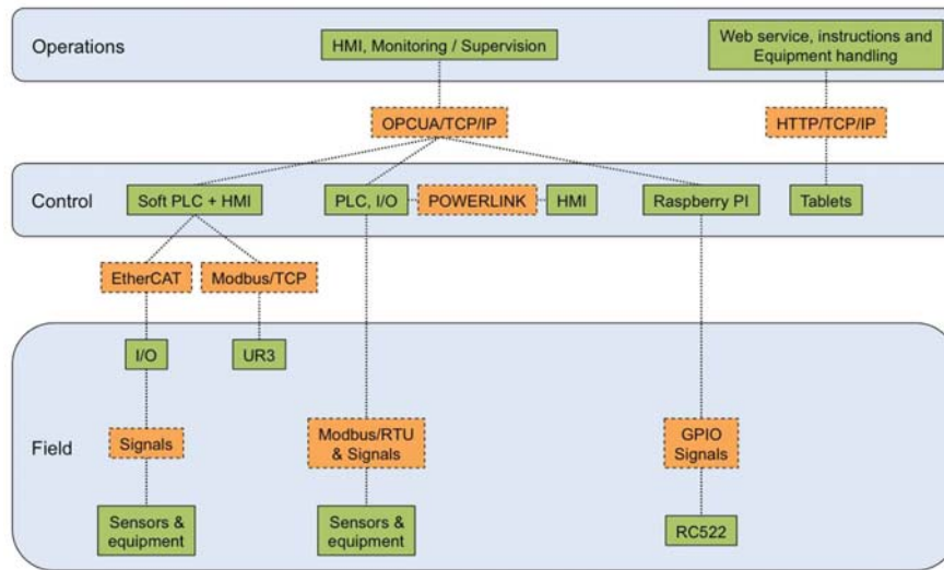
Figure 13: IT system overview of the assembly system (paper II).
