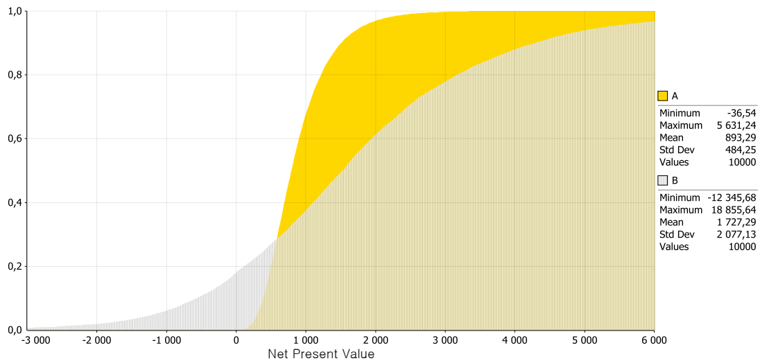
Figure 7 Cumulative probability of alternatives A and B.
