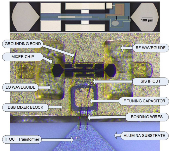
Fig. 4. Interior of ALMA Band 5 DSB SIS mixer. The mixer uses the end-piece configuration (Billade et al. 2013). The Nb-AlOx-Nb SIS junctions have a nominal area of 3 \mu\text{m}^2 , a normal state resistance of R_n = 5 \Omega (for twin-junction configuration Belitsky & Tarasov 1991), a quality factor R_j/R_n \geq 20 , and employ crystal quartz substrates of 90 \mu\text{m} thick. The insert on top shows the details of the Band 5 SIS mixer chip layout to scale. The SIS mixer chips were fabricated by GARD (Pavolotsky et al. 2011) using the Nanofabrication Laboratory Clean room facility at Chalmers University.
