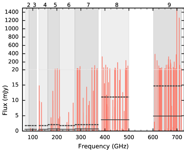
Figure 9. Synthetic spectrum \text{ND}_2\text{H} in the ALMA frequency range. The model assumes T_{\text{ex}} = 200 K, a source size of 0.4 arcsec and a beam of 0.4 arcsec. The numbers at the top indicate the relevant ALMA band. Note the change in scale of the flux around 20 mJy. The solid and dashed lines shows the 1 and 3\sigma levels, respectively.
