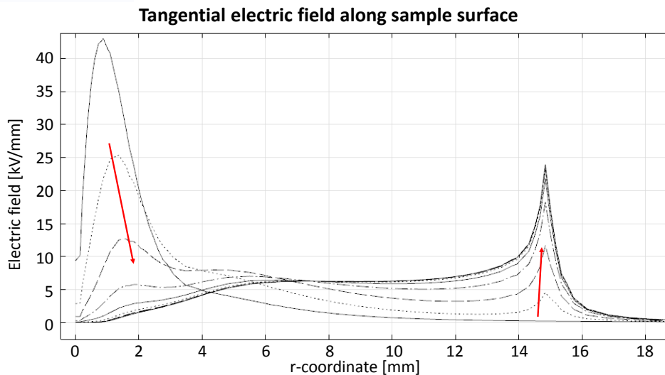
Figure 58. Tangential electric field in DC breakdown test with sample conductivity sweep from 1\text{e-}12\text{ S/m} to 1\text{e-}17\text{ S/m} . Arrows indicate effect of lowering the sample conductivity. The sample edge is located at 15mm.
