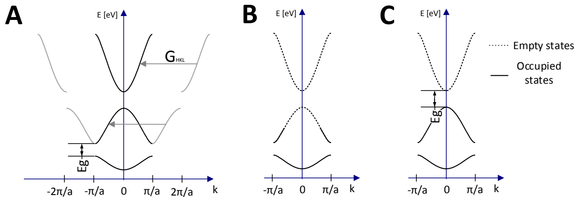
Figure 7. Reduction to reduced zone representation by addition of reciprocal lattice vector (A). E-k diagram for a metal (B). E-k diagram for a semiconductor or insulator with indicated (direct) bandgap E_g (C).
