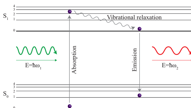
Figure 5.2: Jablonski diagram illustrating the principle of fluorescence. A fluorophore in the ground state S_0 is excited to the higher energy state S_1 upon absorption of the energy of an incoming photon. During relaxation a photon of longer wavelength (lower energy) is emitted.
