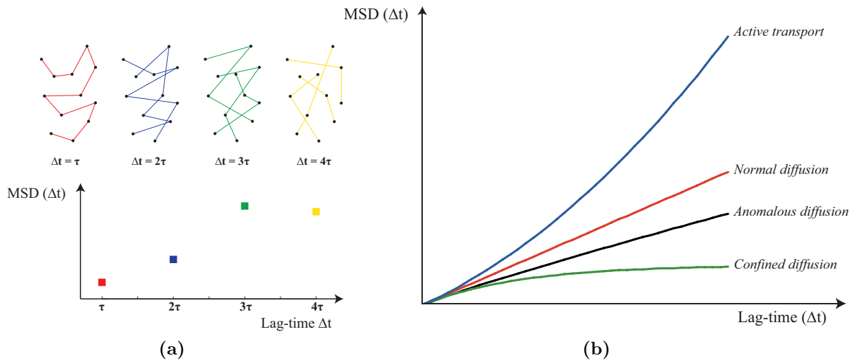
Figure 3.4: Mean squared displacement (MSD), inspired from [80] . (a) Illustration of how an MSD curve is obtained for an arbitrary trajectory and \Delta t = \tau, 2\tau, 3\tau, 4\tau . (b) Different modes of diffusion (active transport, normal diffusion, anomalous diffusion, and confined diffusion) can be determined by the behavior of the MSD curve (see main text for corresponding equations).
