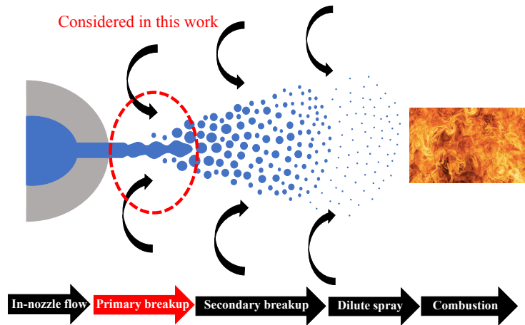
Figure 1.1: Diagram of spray formation
