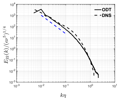
FIG. 1: For homogeneous decaying turbulence at Re_{\lambda} = 155 , normalized DNS and ODT one-dimensional spectra of transverse velocity fluctuations E_{22}(k)/(\epsilon\nu^5)^{1/4} (black lines); (k\eta)^{-5/3} (dashed blue line).
