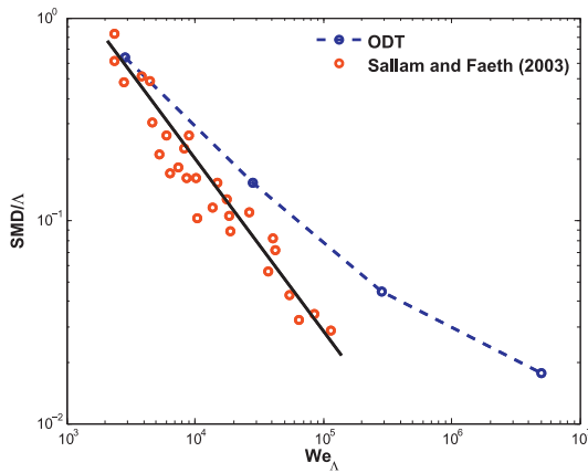
Fig. 9. Droplet diameters at the onset of their formation along the surface of liquid jet as a function of the Weber number.
