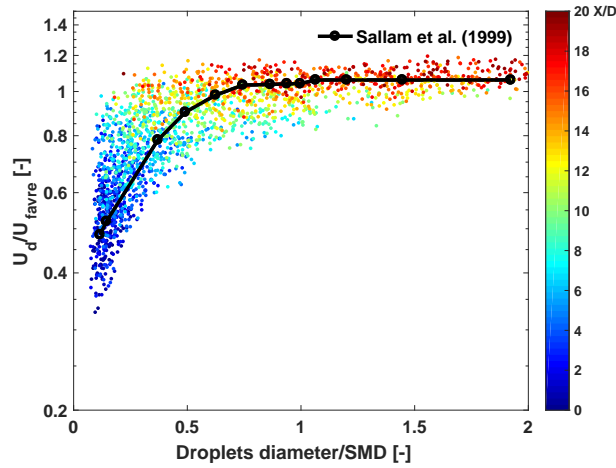
Figure 5.6: Scatter plot of droplet axial velocity, normalized by the Favre velocity, versus diameter. The color indicates the distance from the jet inlet.
