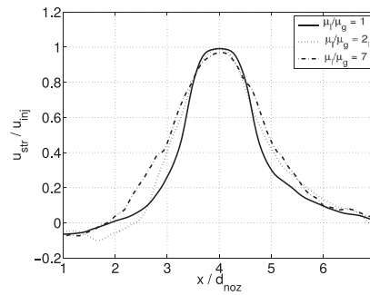
Fig. 11. Average streamwise velocity at a downstream position of z = 30 d_{noz} for different liquid gas viscosity ratio resulting from the VOF simulations. The parameters of the jet are Re_{jet} = 15,000 , We_{jet} = 10,000 and \rho_l/\rho_g = 10 .
