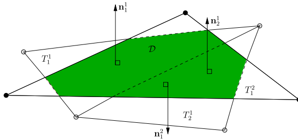
Fig. 2 Triangles from different meshes overlap in a double surface. The double surface is the intersection of triangles $T_1^1$ and $T_2^1$ from one triangle mesh $\mathcal{T}_1$, and triangle $T_1^2$ from a second triangle mesh $\mathcal{T}_2$
