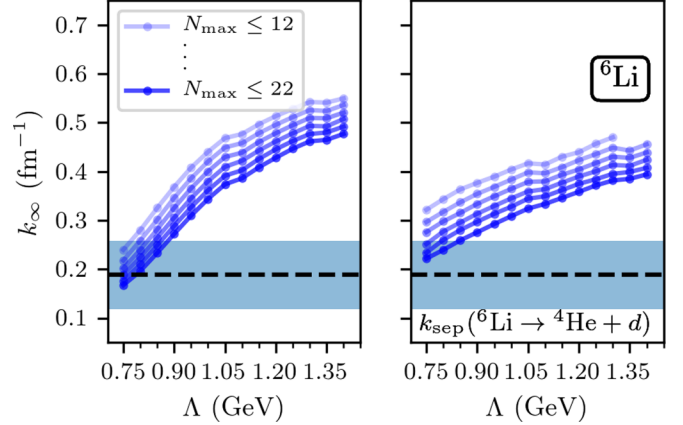
FIG. 16. Fit parameter k_\infty(\Lambda) for {}^6\text{Li} energy extrapolation (left panel) and radius extrapolation (right panel) for different NCSM model space truncations from \max(N_{\max}) = 12 to \max(N_{\max}) = 22 . The lowest, theoretical separation momentum is given as a dashed line with an uncertainty band.
