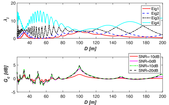
Fig. 3. (Top) Eigenvalues of \mathbf{H}\mathbf{H}^H as a function of D for a 4 \times 4 MIMO with optimized irregular array structure at both TX and RX for D = 100 m; (Bottom) Capacity gain as a function of D .
