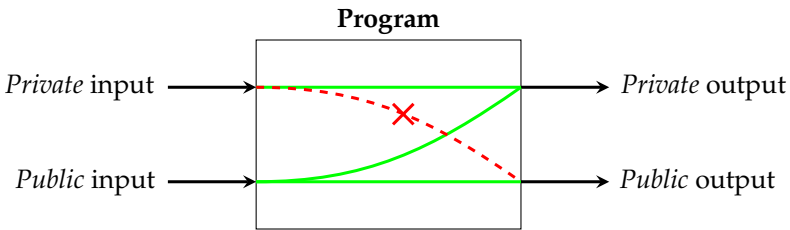
Figure 0.2: Noninterference
