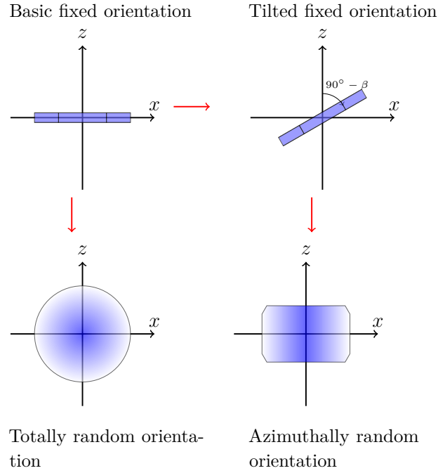
Figure 2.5: A schematic illustration of the difference between totally random (TRO) and azimuthally random orientation (ARO). (Top left) The particle in a fixed state, assumed to be a hexagonal plate (here seen from the side). (Bottom left) The particle in totally random orientation, effectively spherical with decreasing density outwards. (Top right) The particle in a fixed state, but with a tilt angle \beta applied. (Bottom Left) Azimuthally random orientation, i.e. rotation around the z -axis and the particle axis. The particle is effectively symmetric in the horizontal plane.
