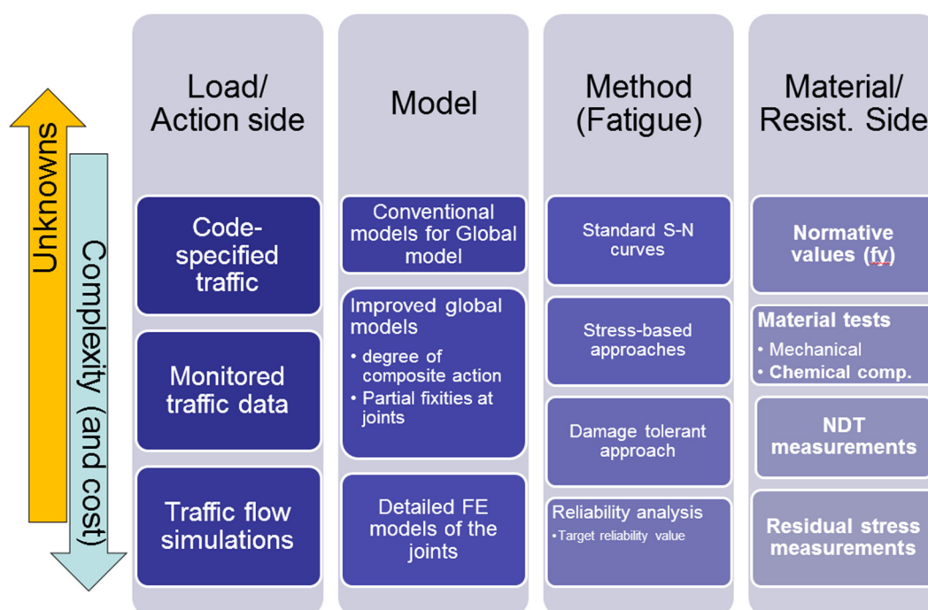
Figure 1.3 Bridge assessment procedures: Increased complexity vs reduced uncertainty.
