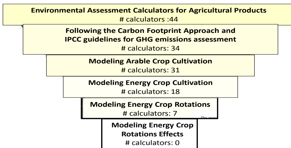
Figure 1 Selection process for GHG emissions calculators for energy crop production 2
