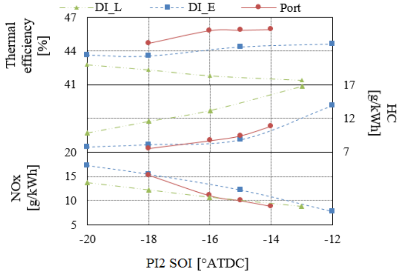
Figure 7.22: Effect of PI2 SOI on thermal efficiency and emissions during methanol-Diesel RCCI combustion
