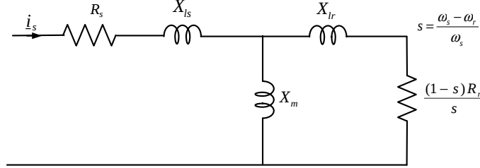
Fig. 2.10 Equivalent circuit of induction machine.
