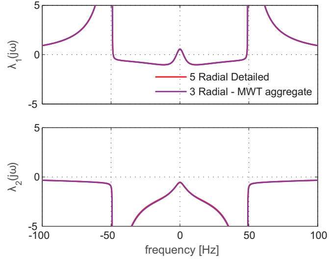
Fig. 4.10 Impact of aggregation using operating condition. Detail model with five radials operated at P_{out} = 0.23 pu, 0.3 pu, 0.6 pu, 0.7 pu and 0.9 pu.(red curve) versus Multiple aggregate model with 3 radials operated at P_{out} = 0.265 pu, P_{out} = 0.6 pu and P_{out} = 0.8 pu
