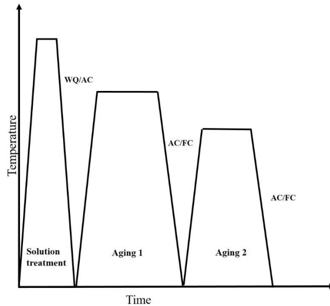
Figure 6 Schematic sketch of heat treatment steps in superalloys
