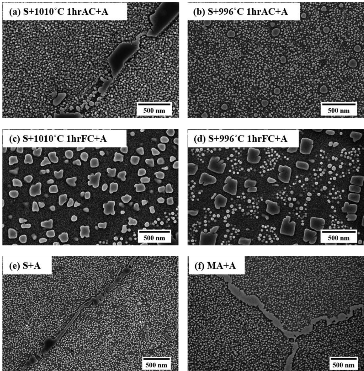
Figure 38 SEM micrographs showing the \gamma' morphology for 1100 °C 60 min WQ solutionised state for different carbide stabilisation conditions as in Table 8.
