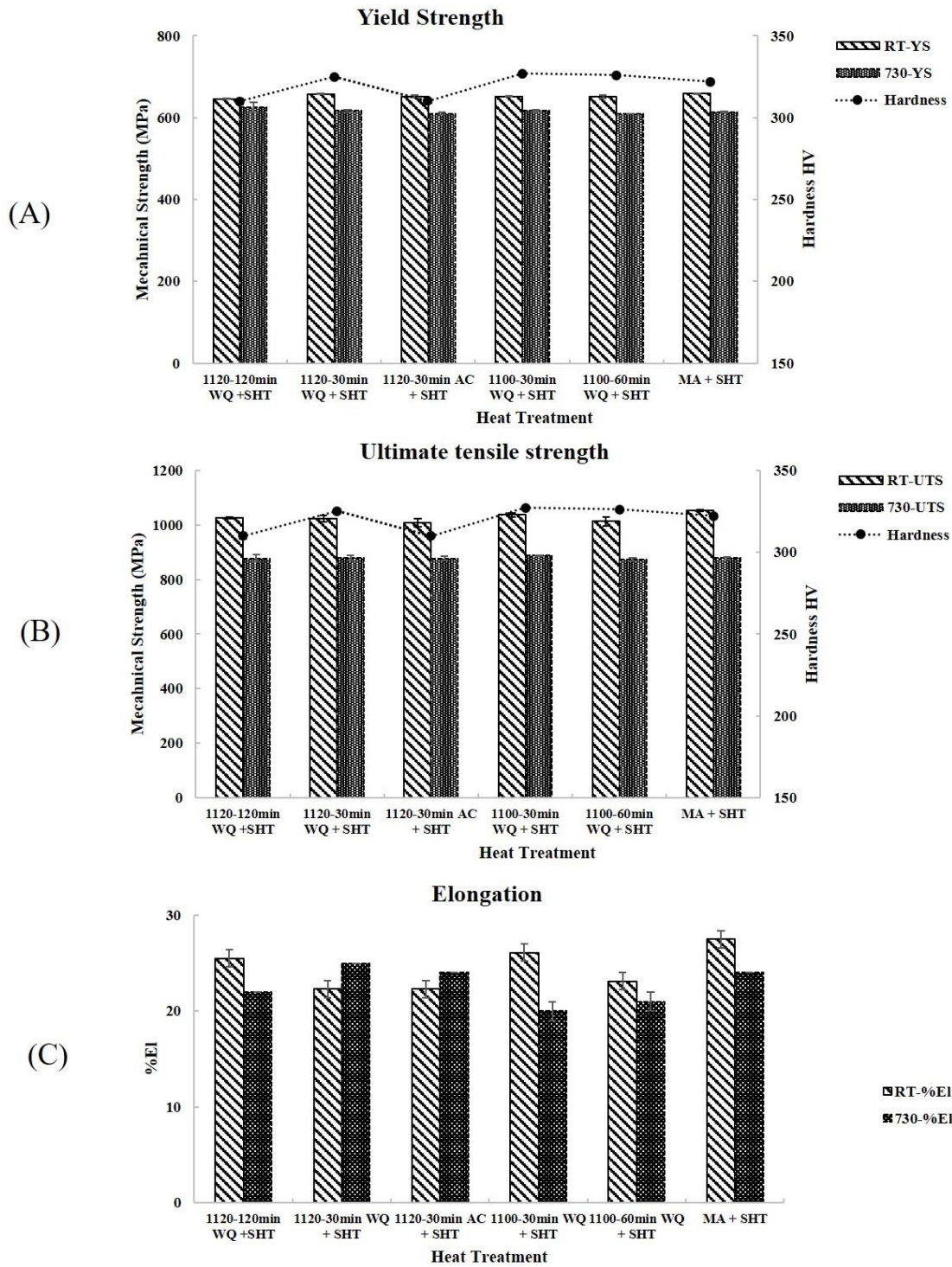
Figure 34 Mechanical properties at 25 and 730 °C for all the heat-treated conditions in Table 6 (a) Yield strength (b) Ultimate tensile strength (c) Elongation.
