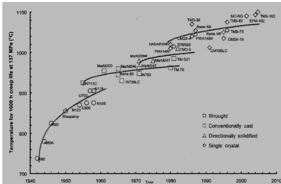
Figure 5 Temperature capability of superalloys since year of introduction [2]
