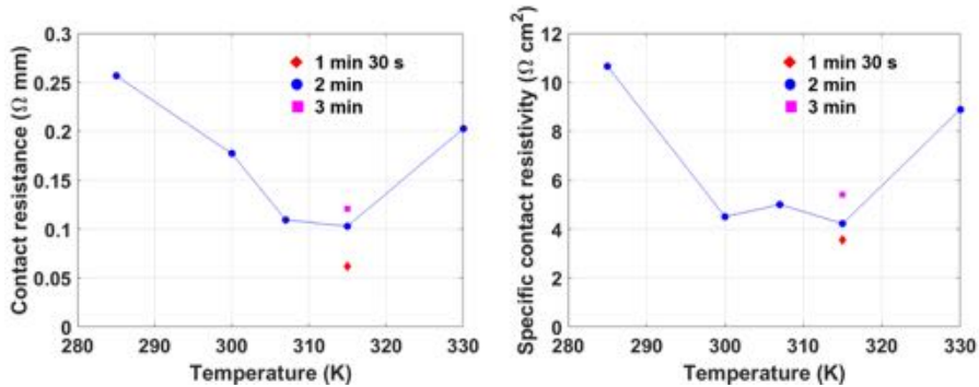
Figure 2.6: Contact resistance measured at 300 K from recessed TLM structures (left) and specific contact resistivity measured from Kelvin structures (right) as a function of annealing temperature.
