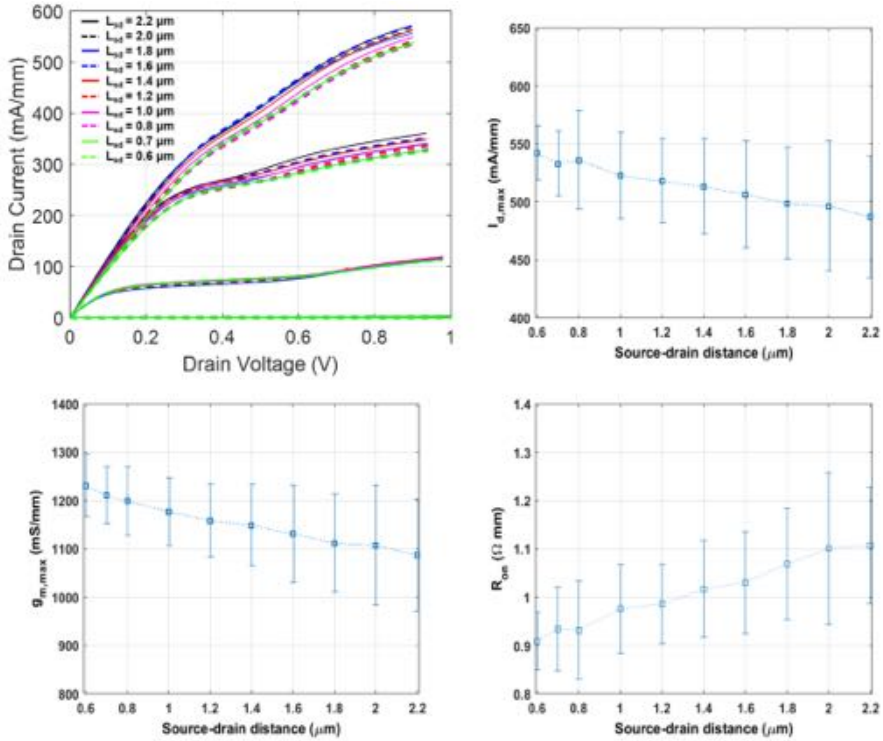
Figure 2.10: The output characteristics of 2 \times 100 \mu\text{m} InP HEMTs at 300 K with L_{sd} ranging from 0.6 \mu\text{m} to 2.2 \mu\text{m} . V_{gs} measured from -0.5 \text{ V} to 0.4 \text{ V} in steps of 0.1 \text{ V} (upper left). The maximum drain current (upper right), maximum transconductance at V_{ds} = 1 \text{ V} (lower left), and on-resistance (lower right) as a function of L_{sd} .
