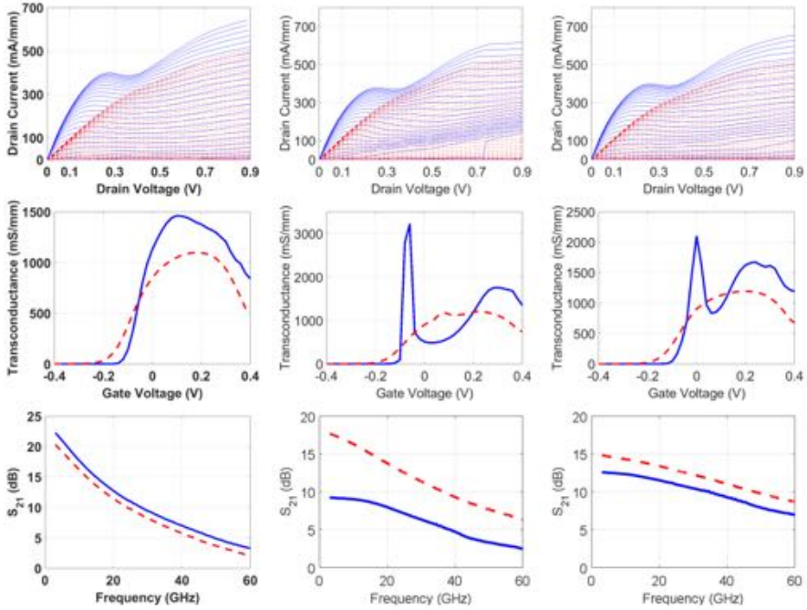
Figure 3.1: The I - V characteristics, transconductance at V_{ds} = 0.8 \text{ V} , and S_{21} at V_{ds} = 0.8 \text{ V} and J_d = 190 \text{ mA/mm} of a 2 \times 100 \mu\text{m} (left column), 2 \times 50 \mu\text{m} (middle column) and 2 \times 30 \mu\text{m} (right column) 100 \text{ nm} HEMTs at 300 \text{ K} (red dashed) and 5 \text{ K} (blue solid).
