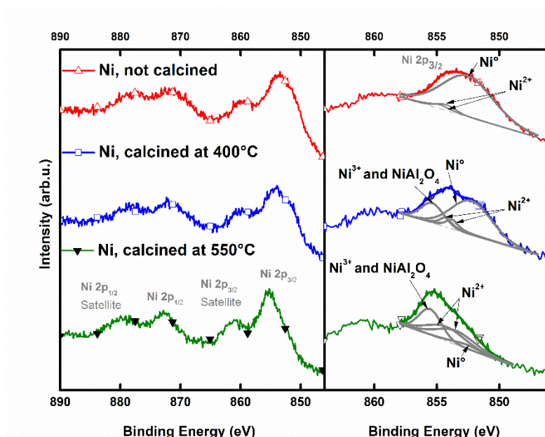
Figure 15. The left panel shows the XPS spectra of three \text{Ni}/\text{Al}_2\text{O}_3 samples for binding energies between 890 and 840 eV, which contain the Ni 2p_{1/2} and Ni 2p_{3/2} and their satellite peak positions. The right panel shows the deconvolution of the Ni 2p_{3/2} peaks.
