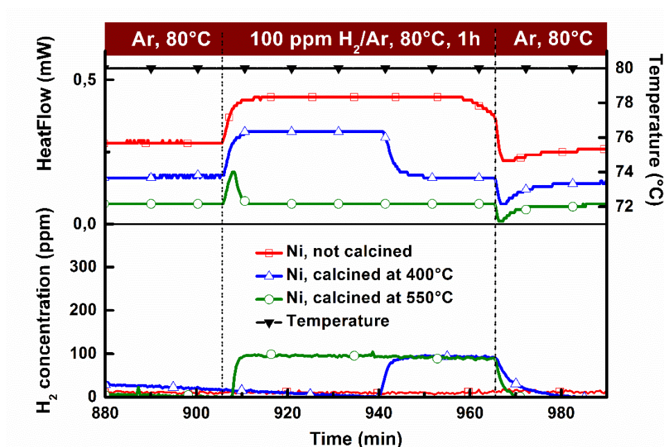
Figure 14. The effect of calcination on the reducibility of Ni/Al 2 O 3 (10 wt%) samples. The top panel shows the heat signal from the DSC and the sample temperature during the adsorption. The bottom panel presents the corresponding hydrogen concentration signal measured by MS.
