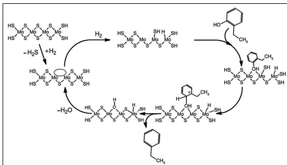
Figure 7. Suggested mechanism of HDO of 2-ethylphenol by a sulfided CoMoS catalyst. The circle indicates the catalytically active vacancy site 149 . Reprinted permission from reference [47].
