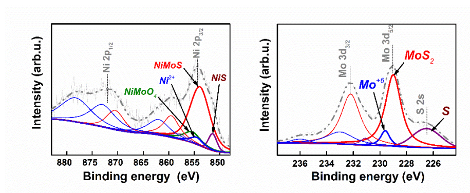
Figure 16. XPS spectra of the Ni 2p, Mo 3d and S 2s core level spectrum for a freshly sulfided sample.
