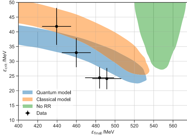
FIG. 9. Experimentally measured \varepsilon_{\text{crit}} as a function of \varepsilon_{\text{final}} measured at the electron spectral feature (points). The shaded areas correspond to the results a hypothetical ensemble of identical experiments would measure 68% of the time under different assumed radiation reaction models for a uniform distribution of a_0 between 4 and 20.
