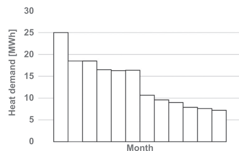
Fig. 1. The figure is showing the distribution of the annual heat demand, including hot tap water and space heating, of the 26 one-family houses in the LEB area in the form of a load duration graph (adapted from (Fahlén et al., 2014)).
