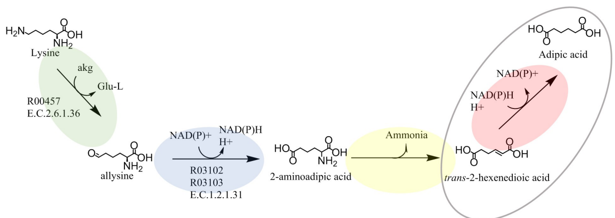
Fig 2. Metabolic pathways for the conversion of lysine to adipic acid. Our alternative pathway. Different types of enzymatic reactions are shown in different colors: removal of NH 2 from \alpha -carbon (yellow), reduction of unsaturated \alpha,\beta bond (pink), removal of the terminal NH 2 (green), and oxidation of aldehyde to carboxylic acid (blue). The enzymatic reactions targeted in this study are encircled. The reaction numbers according to the Kyoto Encyclopedia of Genes and Genomes are given for known reactions. The E.C. numbers according to the Braunschweig Enzyme Database are given for known enzymes. akg = alpha-ketoglutaric acid, Glu-L = L- glutamic acid.
