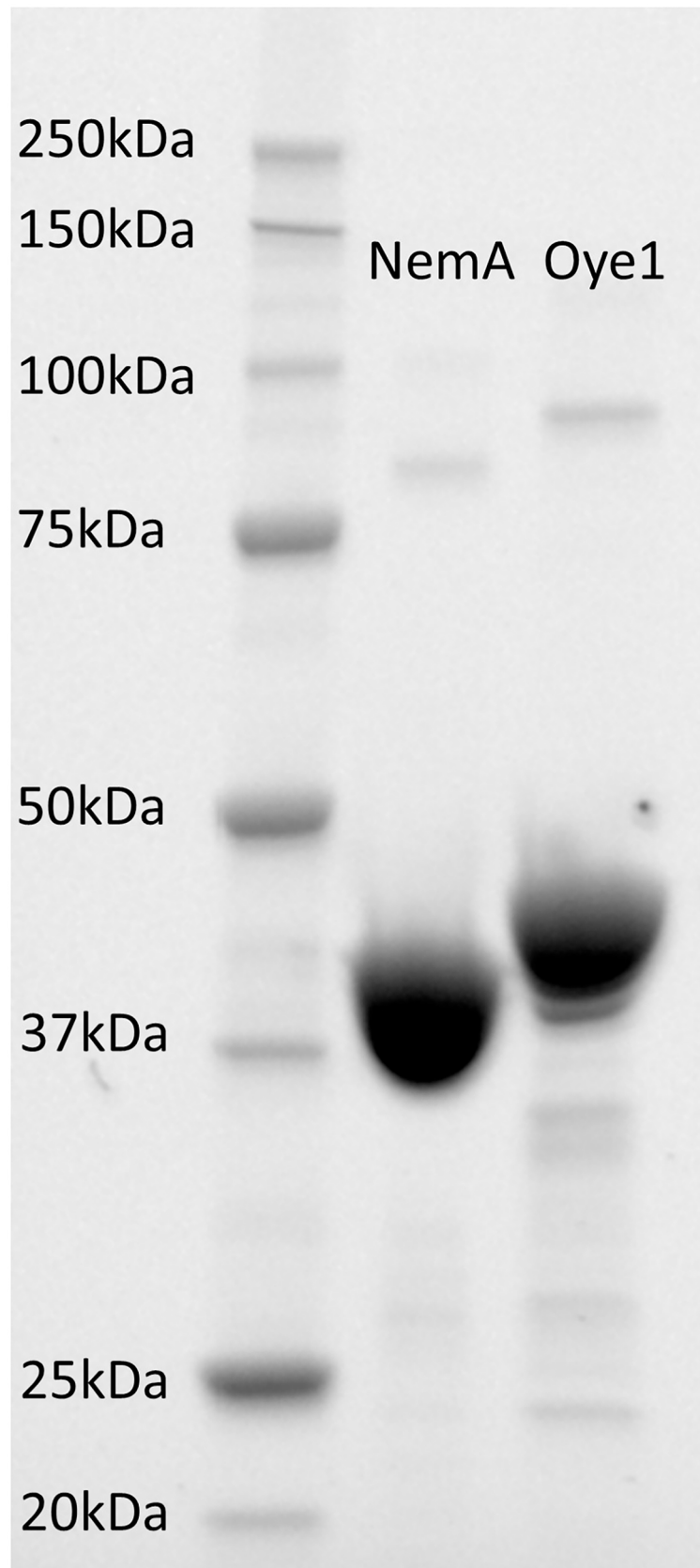
Fig 5. SDS-page separation of the purified enzymes NemaA (43 kDa) and Oye1 (48 kDa).
