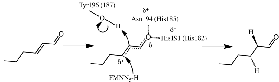
Fig 7. Proposed reaction mechanism of Oye1 and NemA, visualized for the reduction trans -2-hexenal. (Residues in brackets apply to NemA.) Upon hydrogen bonding of the aldehyde to the enzyme (hashed lines) electrons from the double bond are shifted towards the catalytic residues Asn194 (His185) and His191 (His182) (dotted lines), thereby creating a partial positive charge on the \beta -carbon ( \delta^+ ) of the substrate, which activates the double bond and makes it prone to attack. When the double bond is activated the transfer of a hydride from the flavin N_5 to the \beta -carbon of the substrate and protonation from Tyr196 (Tyr187) can occur, resulting in hexanal as the final product. The movement of electrons involved in the hydride attack and protonation are indicated by the curved arrows.
