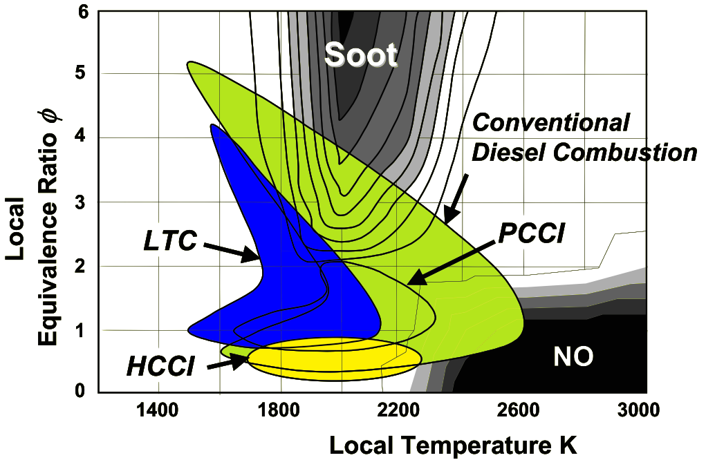
Figure 2: Soot-NOx trade-off for different Diesel combustion regimes adapted from Akihamo [10]
