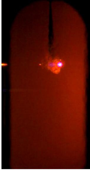
Figure 4: Laser ignition test with pure ethanol
