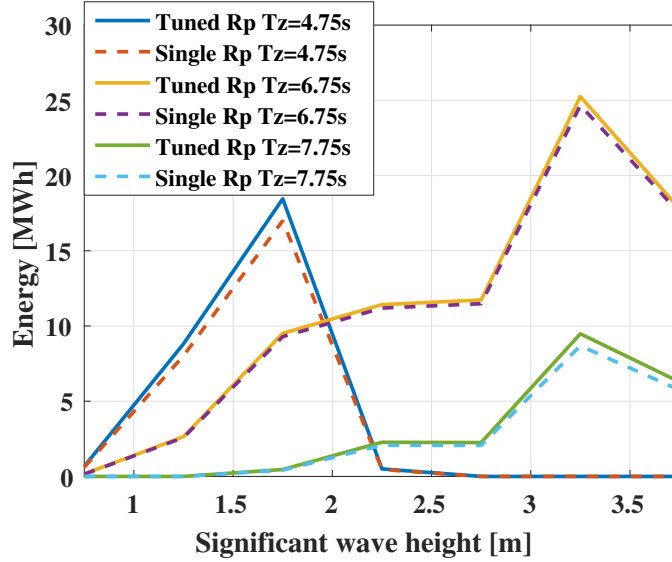
Figure 4.5: Energy differences between the tuned and single R_p for different T_z values.
