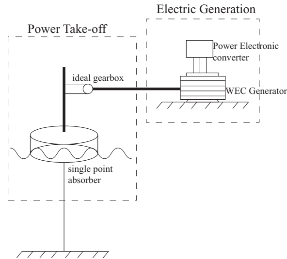
Figure 4.8: An overview of the WEC system.
