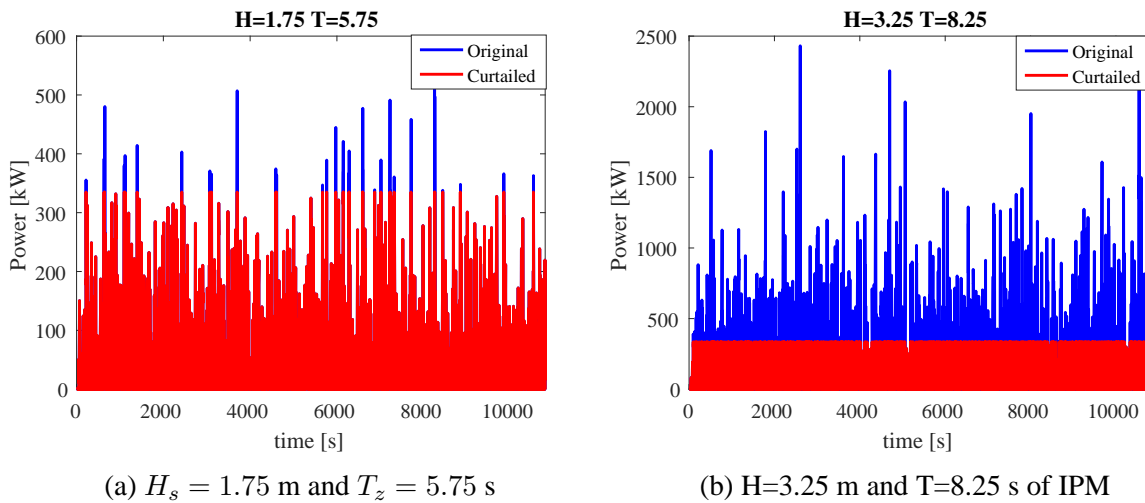
Figure 6.7: Instantaneous power of IPM at different sea states.
