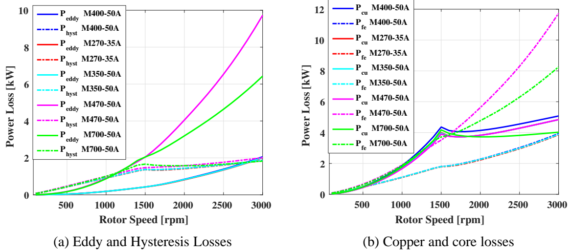
Figure 7.3: Power losses for different steel lamination designs.
