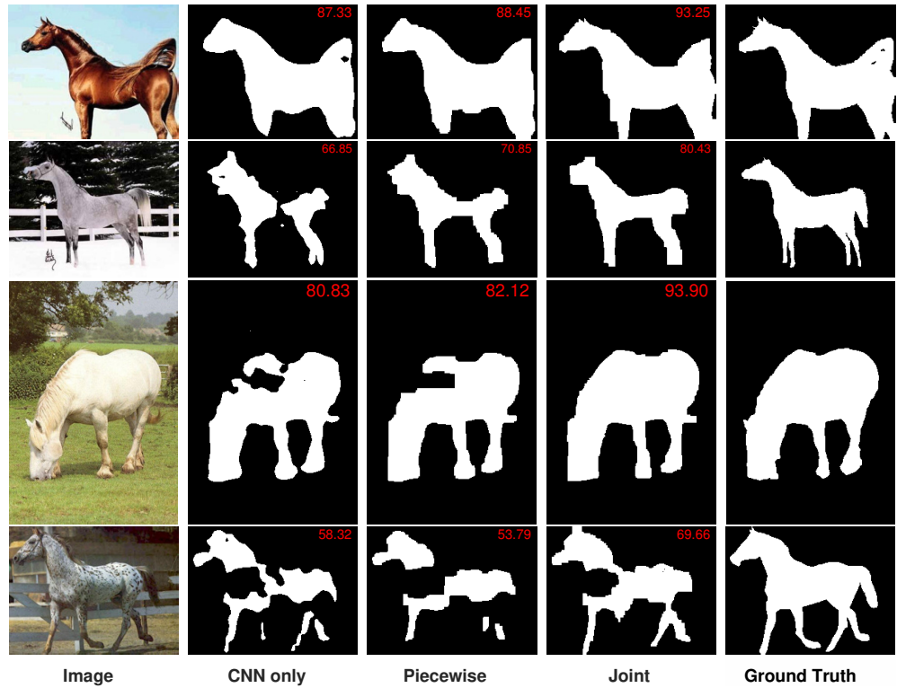
Figure 4: Qualitative results on the Weizmann Horse dataset. "Piecewise" denotes "CNN + CRF (piecewise)" and "Joint" denotes "CNN + CRF (joint)". The red number shown in the upper right corner is the Jaccard index (%). The figure is best viewed in color.
