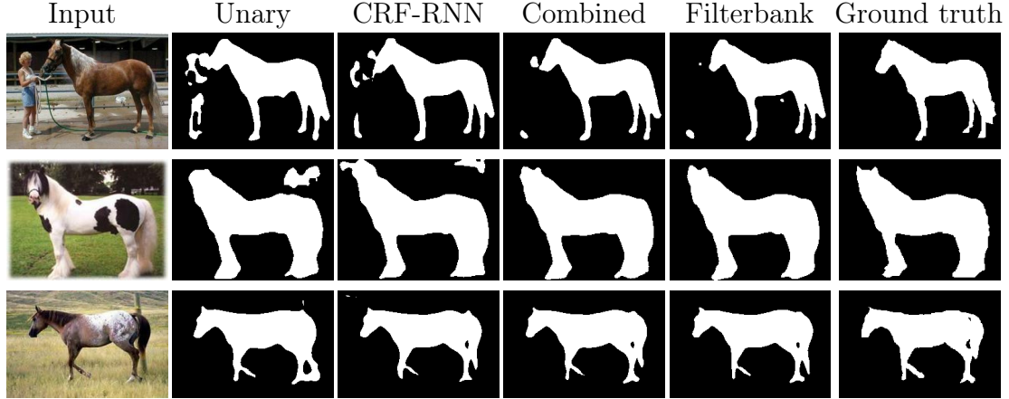
Figure 4: Qualitative results on the WEIZMANN HORSE dataset. Note that the proposed methods capture the shape of the horses better than the baselines, especially compared to the unary network.
