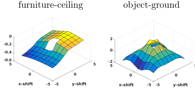
Figure 7: Visualization of the pairwise kernel weights for the filterbank version trained on the NYU V2 data set. These weights are for the classes shown above the plots and for the third filter choosing map which usually has a high value for pixels with no semantic edge. The furniture-ceiling kernel favors putting furniture labels below ceiling labels while the object-ground kernel has a more Gaussian-like shape.
