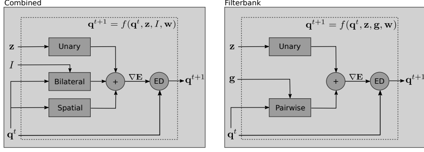
Figure 1: The data flow of one iteration of the projected gradient descent algorithm. Each rectangle or circle represent an operation that can be performed within a deep learning framework, the ED component performs an entropic descent update step according to equation (13). Left: Combined version of CRF, Right: Filterbank version of CRF.
