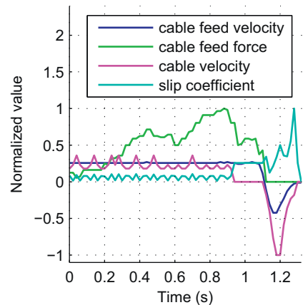
Fig. 17. (a) Normalized values of the cable feed wheels' velocity, the supervised cable feed force, the supervised cable gripping force and the calculated force slip coefficient during a feed-to-slip operation where the slip coefficient limit was adjusted to 1 and the velocity slip supervision was inactivated, with measurement sampling frequency 50 Hz. For reference, the actual maximum absolute values shown in the figure are 228 mm/s velocity and 405 N force. (b) Normalized values of the cable feed wheels' velocity, the supervised cable feed force, the supervised cable velocity and the calculated velocity slip coefficient during a feed-to-slip operation. Here, the slip detection time was adjusted to 0.1 s, a cable gripping force of about 75 N was used and the force slip supervision was inactivated. The measurement sampling frequency was 50 Hz. For reference, the actual maximum absolute values shown in the figure are 84 N force and 78 mm/s velocity.
