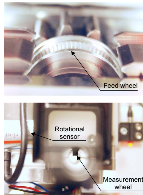
Fig. 7. (a) A feed wheel mounted with a cog wheel inside a robot cable feeder tool. (b) The measuring wheel of the miniature cable fed distance measuring system, as seen from the cable guiding system end of a robot cable feeder tool.
