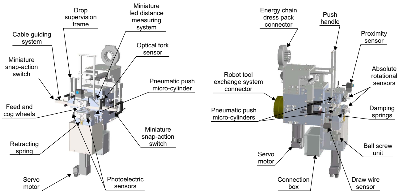
Fig. 5. A 3D-CAD model explaining the most essential parts of the updated robot cable feeder tool design.
