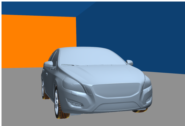
(b) Vehicle representation in the numerical domain
