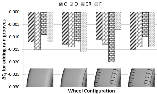
(b) Overall C_l change
