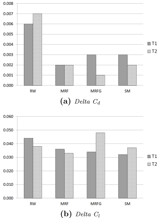
Figure 2.10: Changes in C_d and C_l of the vehicle when using different modelling methods for tyre rotation on a closed rim and referenced to T_0
