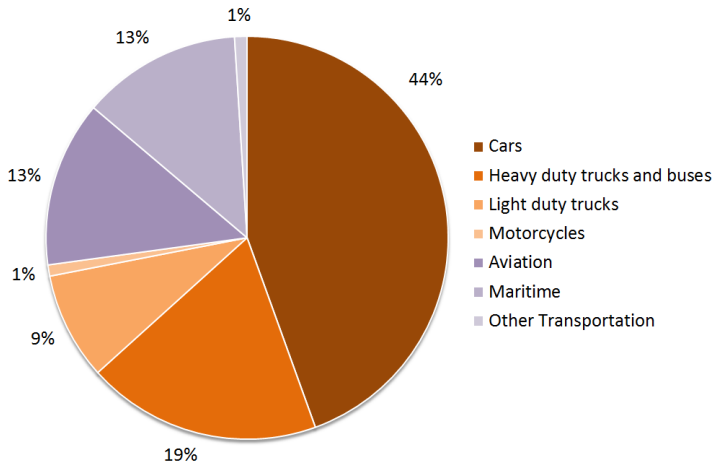
Figure 1.2: CO 2 emissions in Europe 2014 from different sectors [7].
