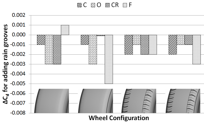
(a) Overall C_d change
