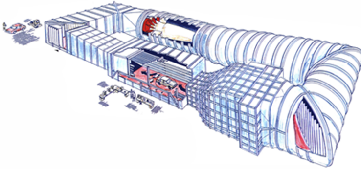
Figure 3.4: Volvo Cars Aerodynamic Wind Tunnel
