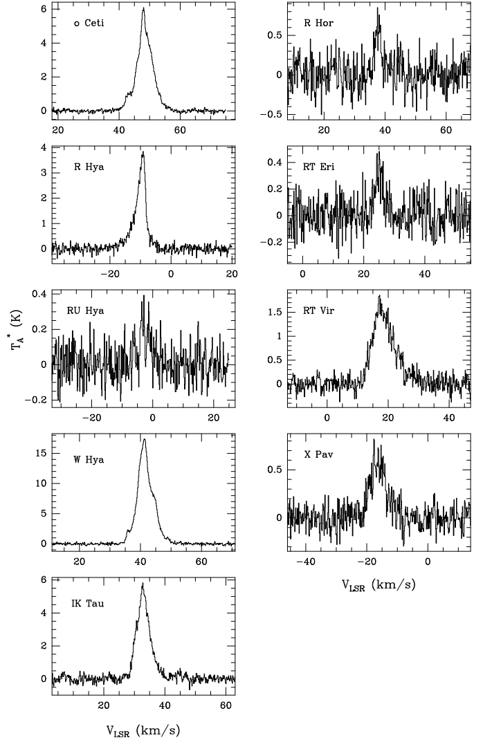
Fig. 1. Spectra of the (0, 1, 0), J = 1_{1,0}-1_{0,1} transition of water at 658 GHz toward nine Mira-type or semi-regular variables in our sample. The antenna temperature is for outside the atmosphere and the spectral resolution is 0.14 km s -1 for all sources. See Sect. 2.3 for Jy to K conversion at the time of the observations.
