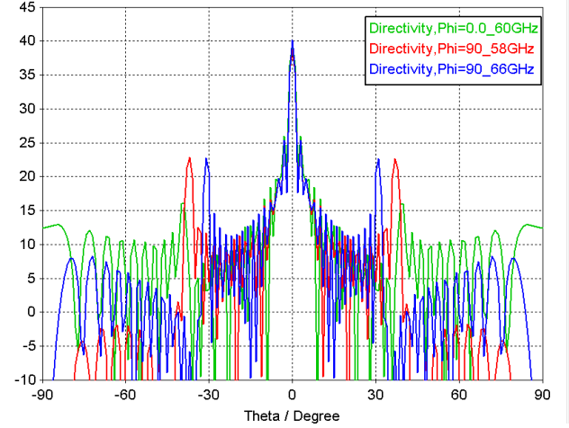
Fig. 5(a) H-plane pattern for the 32 \times 32 element array.
