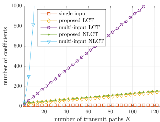
Figure 5.4. Illustration of how the number of coefficients per transmit path scales with the number of paths. The figure shows the number of DPD coefficients per switching region plus the number of CTMM coefficients. Numbers are shown for: single-input DPD; the proposed DPD and multi-input DPD based on models with linear crosstalk terms indicated by LCT; the proposed DPD and multi-input DPD based on models using linear and nonlinear terms of the crosstalk signals indicated by NLCT.
