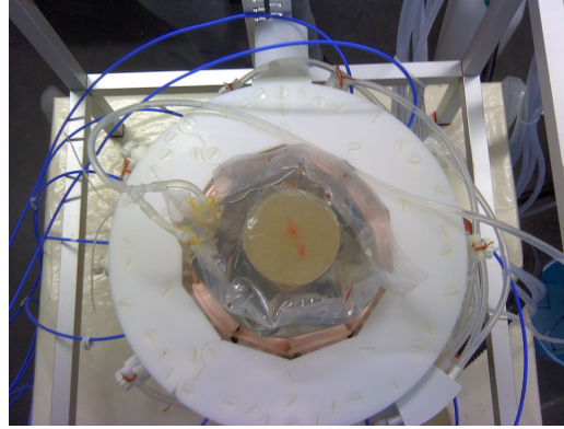
Figure 4.2: Measurement setup shows the muscle phantom surrounded by water bag and applicator.
