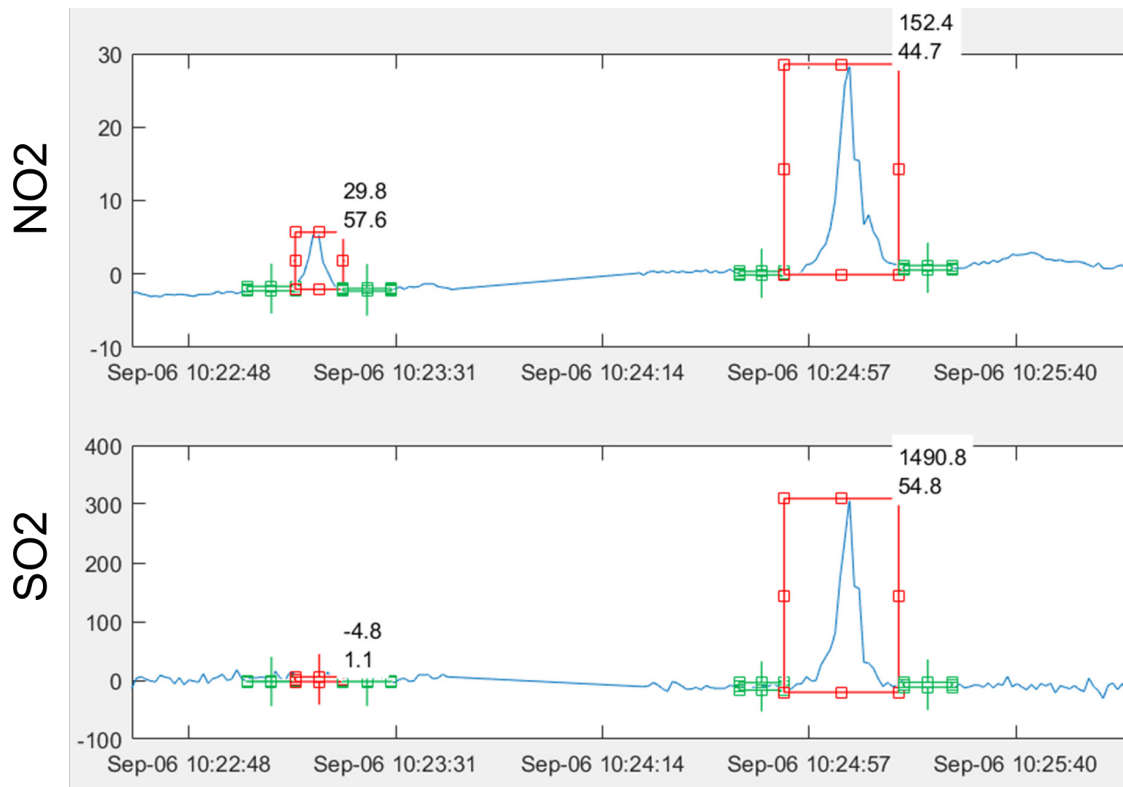
Figure 3. Optical measurements of \text{NO}_2 and \text{SO}_2 of two ships, one running on 0.1 % m/m fuel and another one running on 1 % m/m fuel is shown. The data were obtained at the SECA border as part of the CompMon project (Mellqvist et al., 2017 a).
