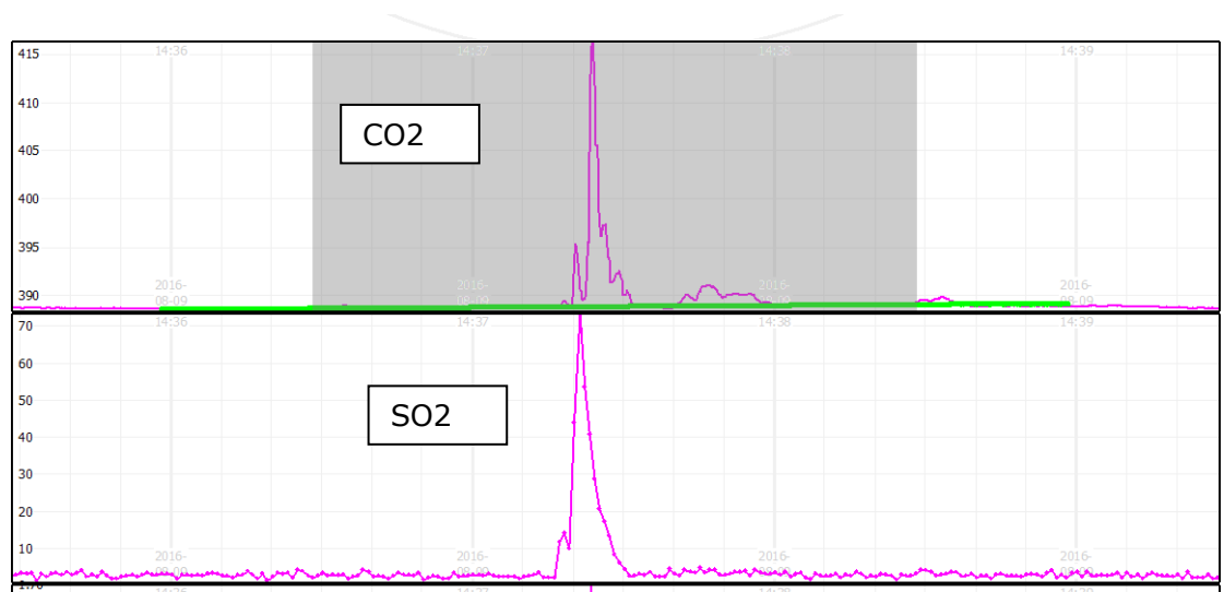
Figure 28. A quality assurance test in which a short pulse (10s) of premixed \text{SO}_2 and \text{CO}_2 gas was blown across the airplane inlet and analyzed by the sniffer systems in the aircraft. Here is shown the concentration of \text{CO}_2 (top) in ppm and \text{SO}_2 (middle) in ppb versus time.
