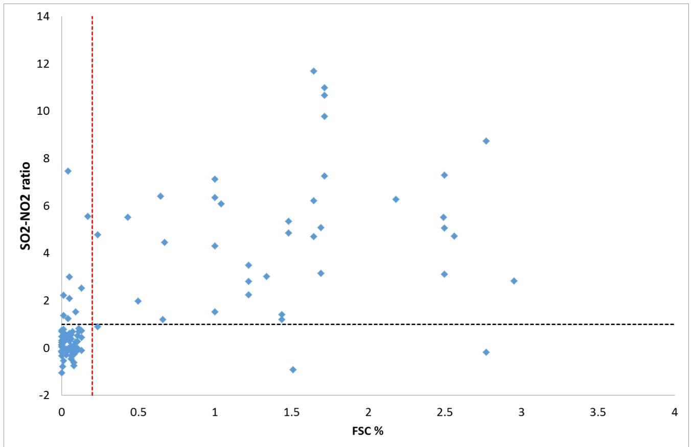
Figure 4. The measured ratio of \text{SO}_2 and \text{NO}_2 from the optical sensor and the FSC obtained from sniffer measurements. The data were obtained in the CompMon project at the SECA border (Mellqvist et al., 2017a).
