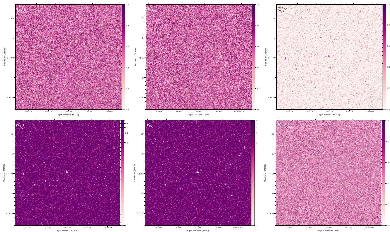
Figure 7. Similar simulated images as those shown in Fig. 5, but showing the outputted p -values from the skewness (top row) and excess kurtosis (bottom row) tests. Images are shown for the Q (left column), U (middle column), and P (right column) data. The excess kurtosis p -value images are particularly useful indicators of the presence of polarized sources.
