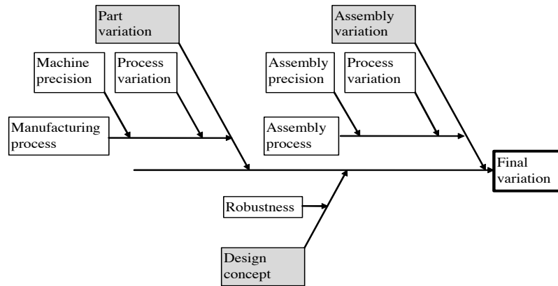
Figure 13 Contributors to final geometrical variation by (Söderberg, 1998)
