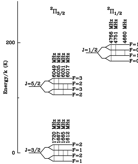
Figure 1.2: Energy diagram showing the ground and two first excited rotational states of OH. The \Lambda -doubling and hyperfine levels are not to scale. Transitions between hyperfine levels are indicated with lines connecting the levels in question and their frequencies are shown above the lines.
