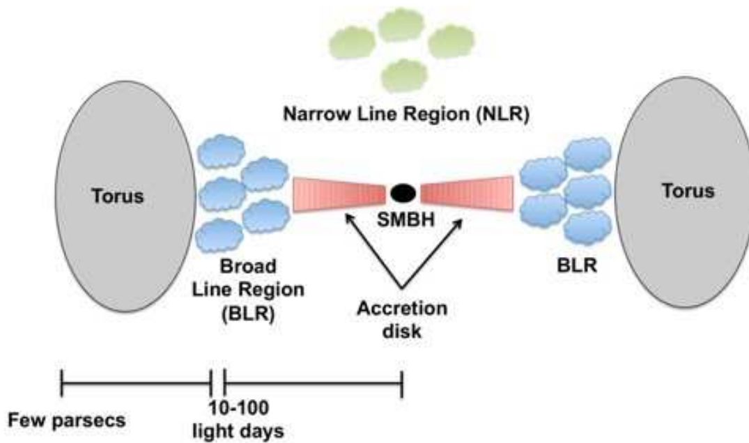
Figure 2.1: Schematic view of the structure of an AGN in the unification models. The class of AGN seen depends on the viewing angle with respect to the torus. Credit: Claudio Ricci - http://www.isdc.unige.ch/~ricci/Website/Active_Galactic_Nuclei.html
