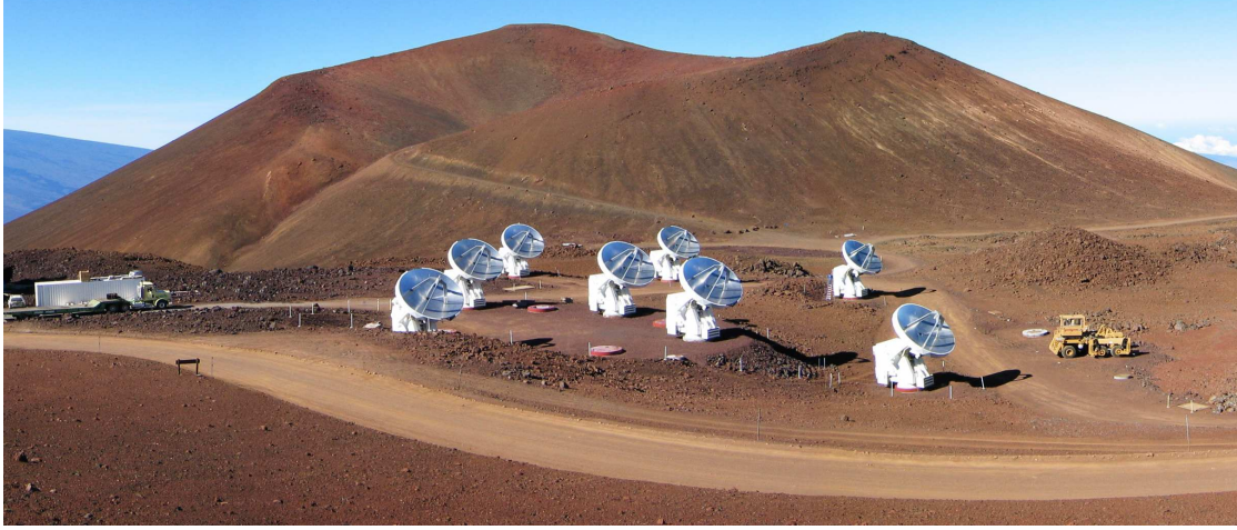
(a) View of the eight antennas of the SMA. Credit: J. Weintraub
