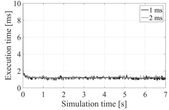
Figure 9. Real-time execution times per time step with 1ms and 2ms time steps. Each time step takes the same amount of time regardless of the length of the timestep.
