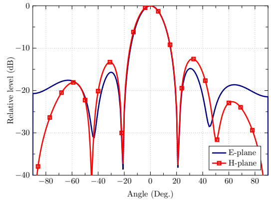
Fig. 5. x-direction polarization
