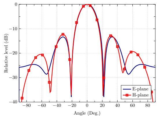
Fig. 6. y-direction polarization
